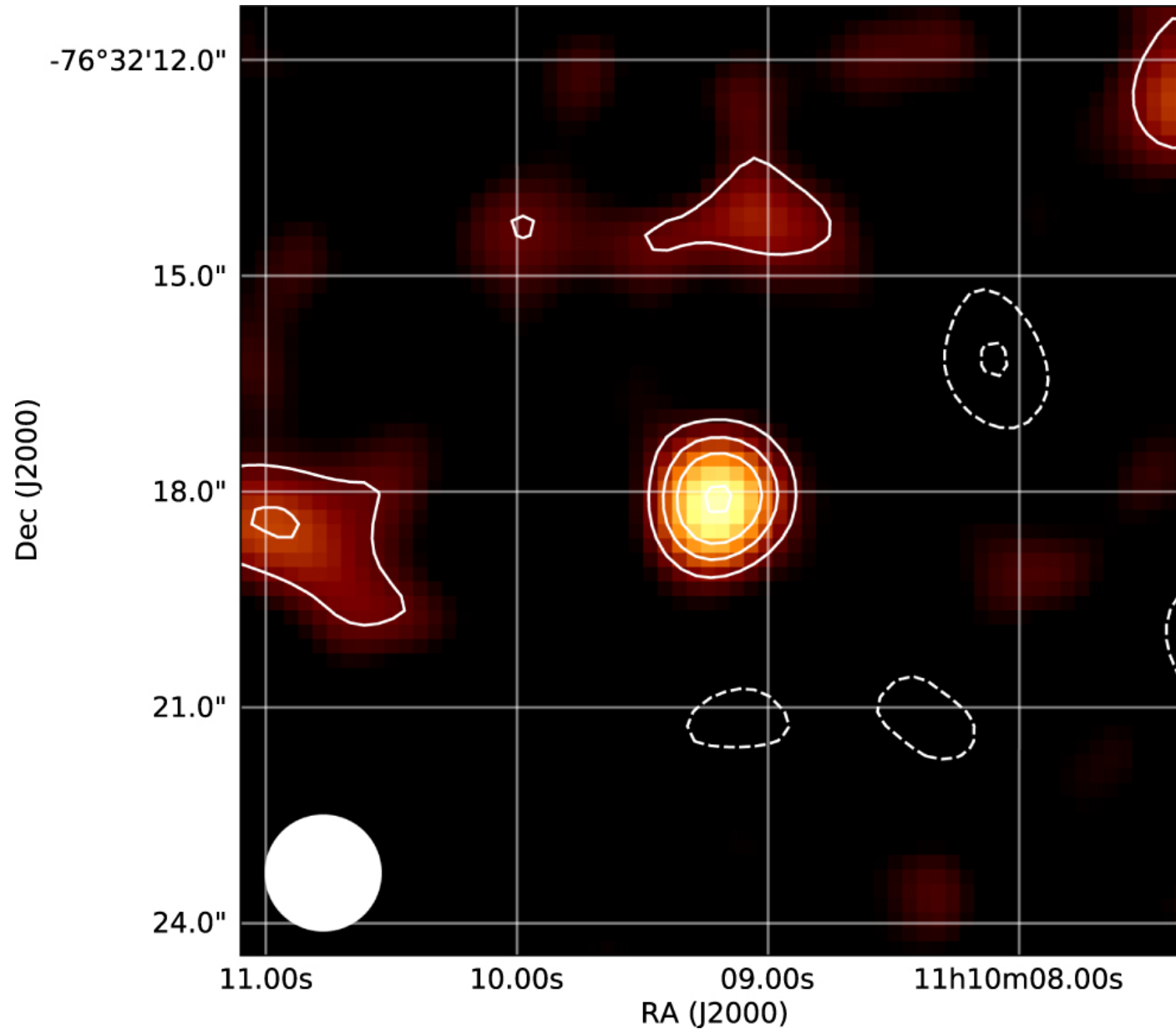
Figure 1. from First Millimeter Detection of the Disk around a Young, Isolated, Planetary-mass Object null 2017 APJL 841 L11 doi:10.3847/2041-8213/aa7046 https://dx.doi.org/10.3847/2041-8213/aa7046 © 2017. The American Astronomical Society. All rights reserved.
