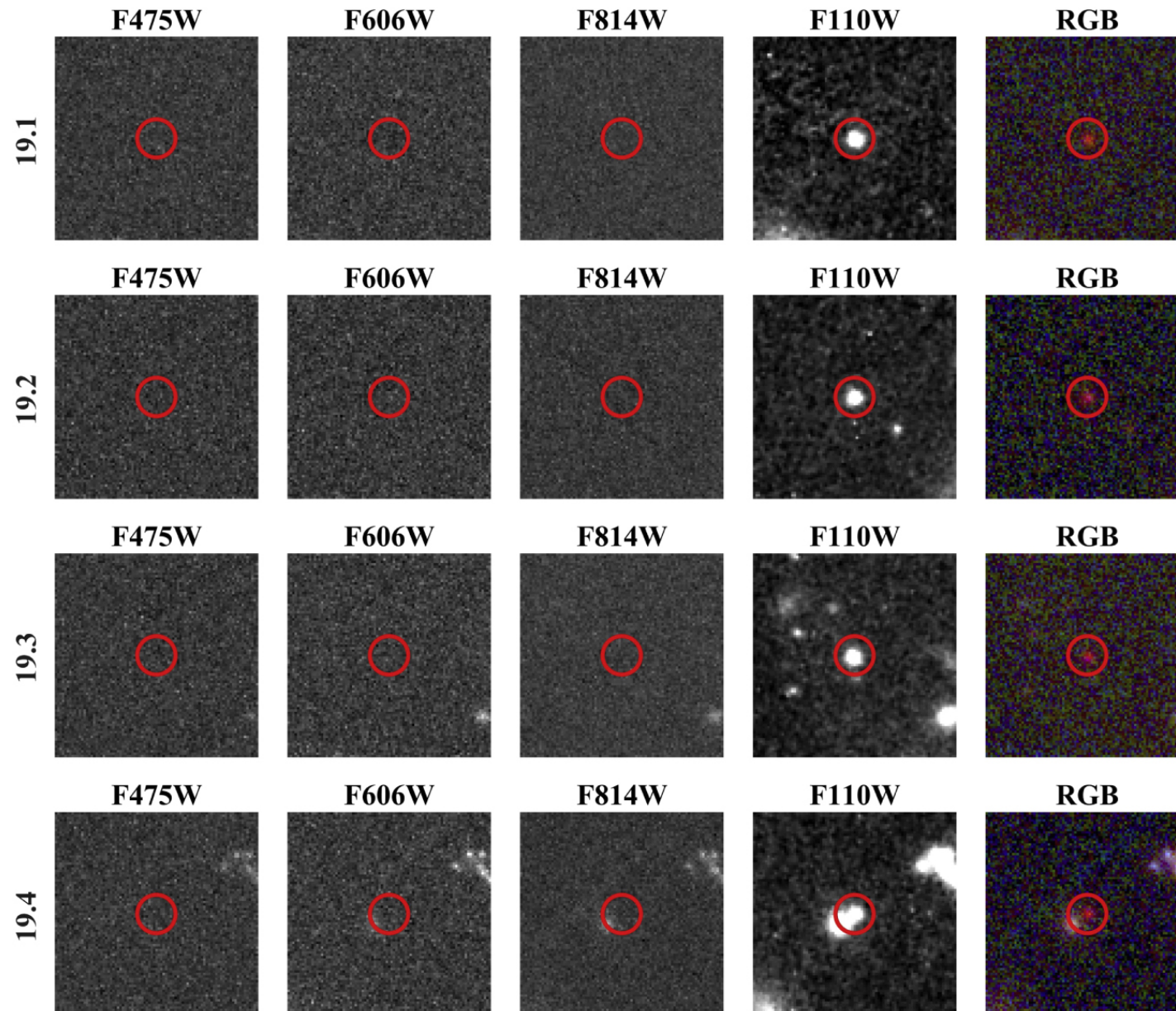
Figure 4. from A Very Large (E 40) Strong Gravitational Lens Selected with the Sunyaev–Zel’dovich Effect: PLCK G287.0+32.9 ( z = 0.38 ) null 2017 APJL 839 L11 doi:10.3847/2041-8213/aa69be https://dx.doi.org/10.3847/2041-8213/aa69be © 2017. The American Astronomical Society. All rights reserved.
