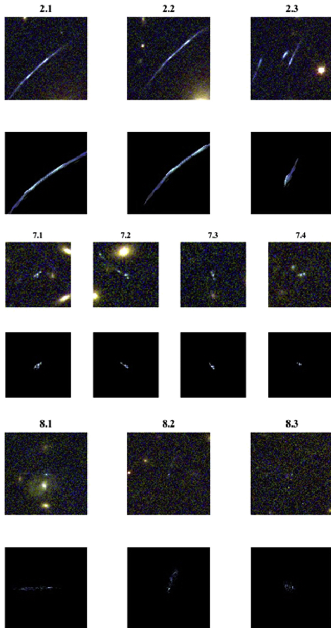
Figure 3. from A Very Large (E 40) Strong Gravitational Lens Selected with the Sunyaev–Zel’dovich Effect: PLCK G287.0+32.9 ( z = 0.38 ) null 2017 APJL 839 L11 doi:10.3847/2041-8213/aa69be https://dx.doi.org/10.3847/2041-8213/aa69be © 2017. The American Astronomical Society. All rights reserved.
