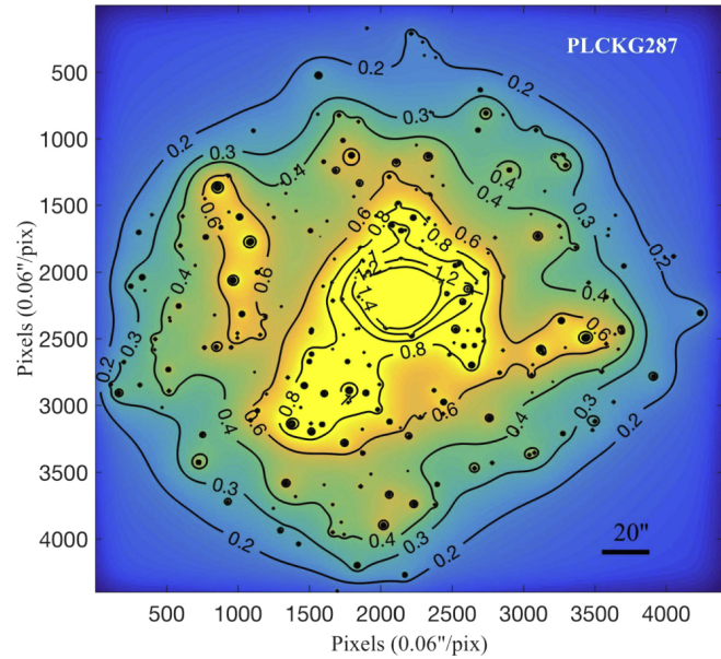
Figure 2. from A Very Large (E 40) Strong Gravitational Lens Selected with the Sunyaev–Zel’dovich Effect: PLCK G287.0+32.9 ( z = 0.38 ) null 2017 APJL 839 L11 doi:10.3847/2041-8213/aa69be https://dx.doi.org/10.3847/2041-8213/aa69be © 2017. The American Astronomical Society. All rights reserved.
