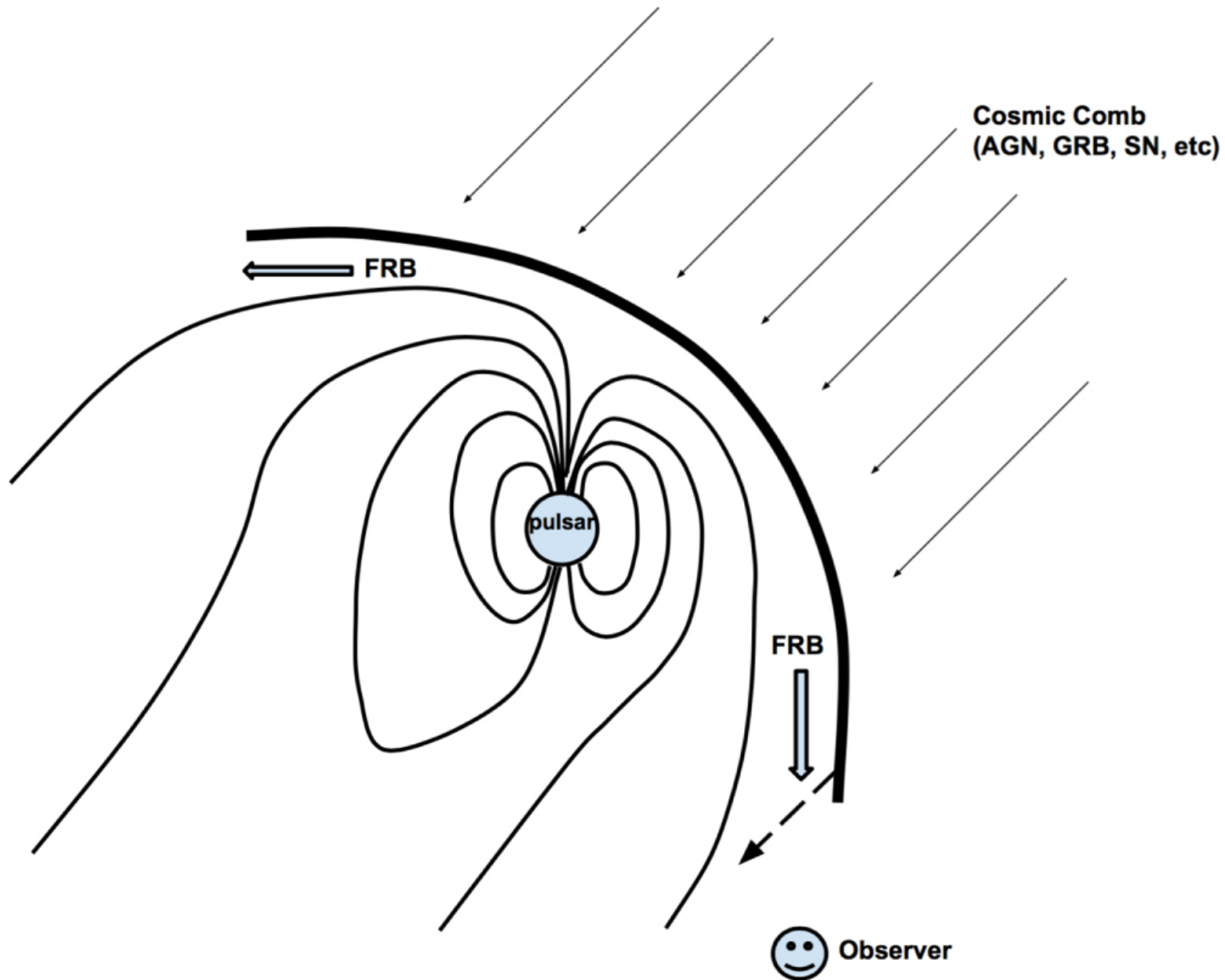
Figure 1. from A “Cosmic Comb” Model of Fast Radio Bursts null 2017 APJL 836 L32 doi:10.3847/2041-8213/aa5ded https://dx.doi.org/10.3847/2041-8213/aa5ded © 2017. The American Astronomical Society. All rights reserved.
