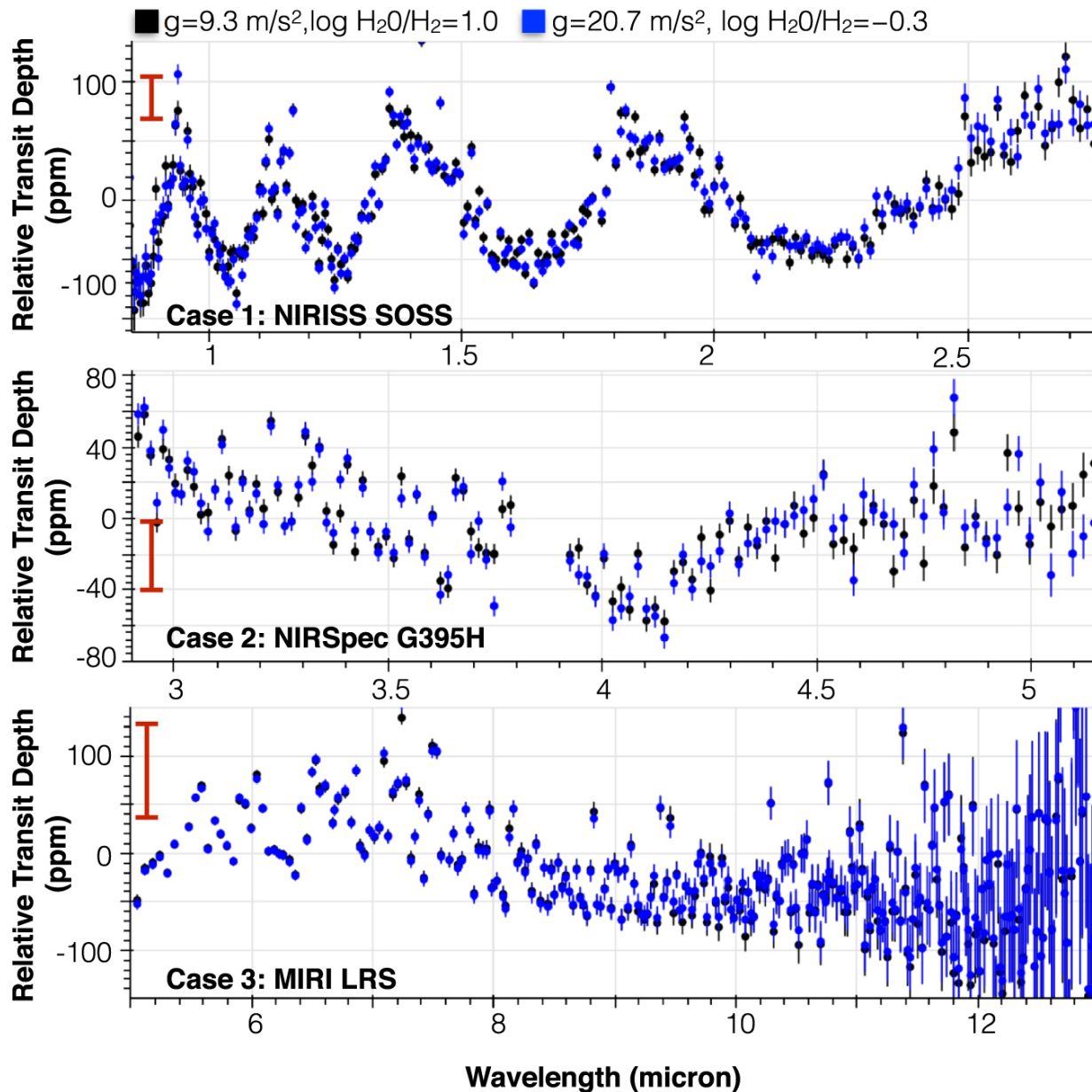
Figure 2. from Challenges to Constraining Exoplanet Masses via Transmission Spectroscopy null 2017 APJL 836 L5 doi:10.3847/2041-8213/aa5c7d https://dx.doi.org/10.3847/2041-8213/aa5c7d © 2017. The American Astronomical Society. All rights reserved.
