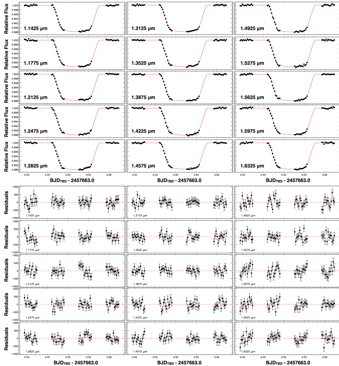
Figure 2. from HST PanCET Program: A Cloudy Atmosphere for the Promising JWST Target WASP-101b null 2017 APJL 835 L12 doi:10.3847/2041-8213/835/1/L12 https://dx.doi.org/10.3847/2041-8213/835/1/L12 © 2017. The American Astronomical Society. All rights reserved.
