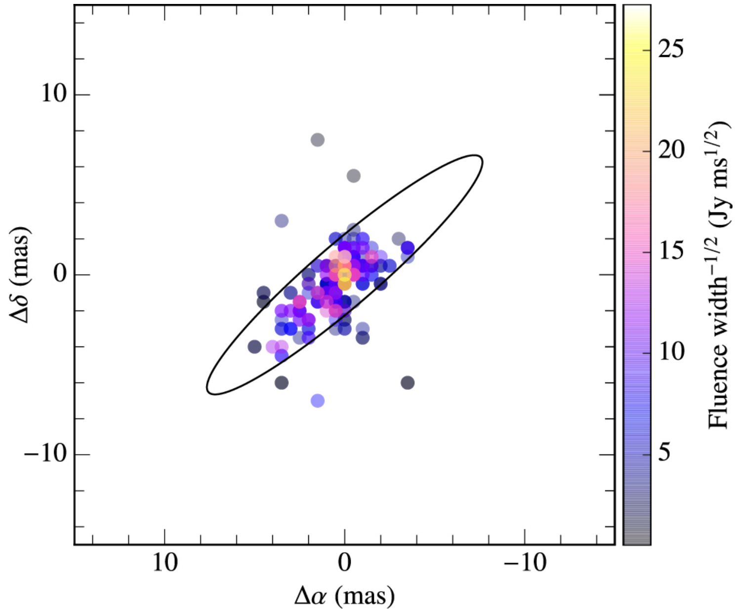
Figure 4. from The Repeating Fast Radio Burst FRB 121102 as Seen on Milliarcsecond Angular Scales null 2017 APJL 834 L8 doi:10.3847/2041-8213/834/2/L8 https://dx.doi.org/10.3847/2041-8213/834/2/L8 © 2017. The American Astronomical Society. All rights reserved.
