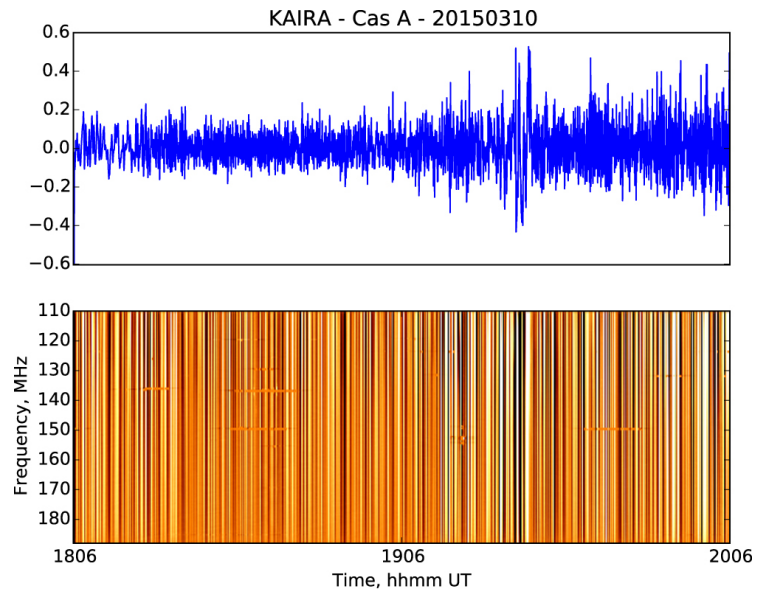
Figure 5. from SEPARATING NIGHTSIDE INTERPLANETARY AND IONOSPHERIC SCINTILLATION WITH LOFAR null 2016 APJL 828 L7 doi:10.3847/2041-8205/828/1/L7 https://dx.doi.org/10.3847/2041-8205/828/1/L7
