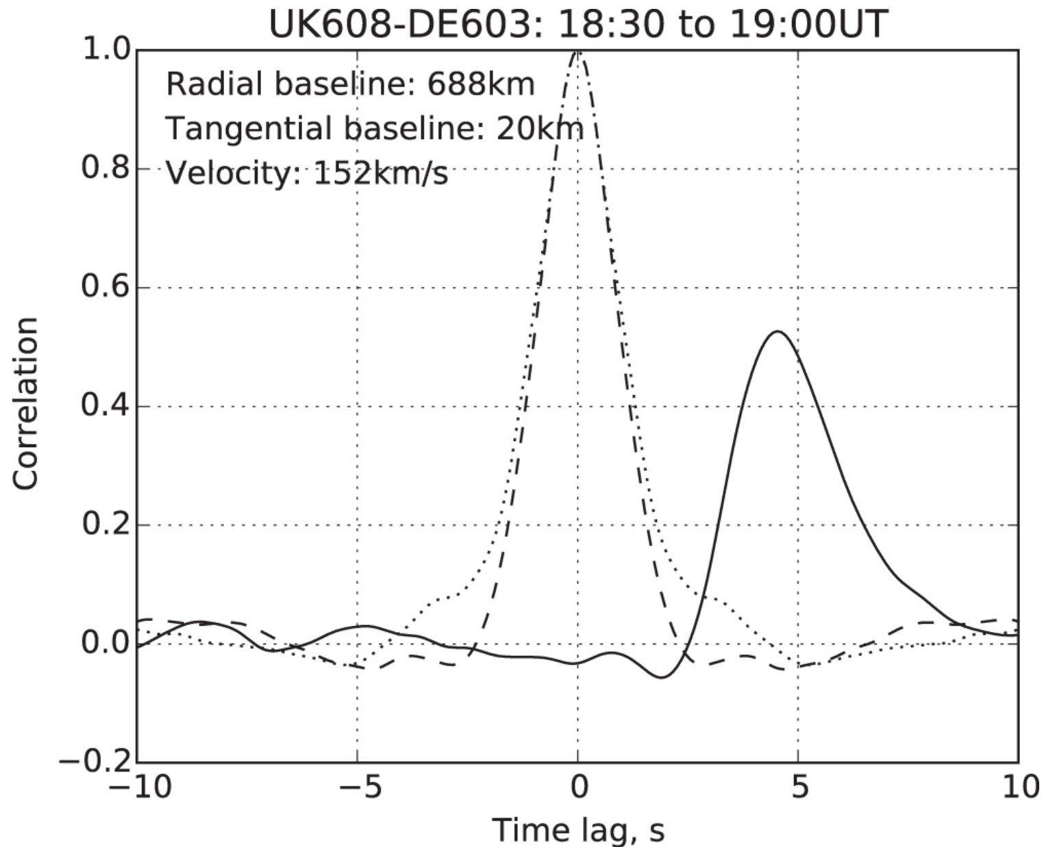
Figure 4. from SEPARATING NIGHTSIDE INTERPLANETARY AND IONOSPHERIC SCINTILLATION WITH LOFAR null 2016 APJL 828 L7 doi:10.3847/2041-8205/828/1/L7 https://dx.doi.org/10.3847/2041-8205/828/1/L7 © 2016. The American Astronomical Society. All rights reserved.
