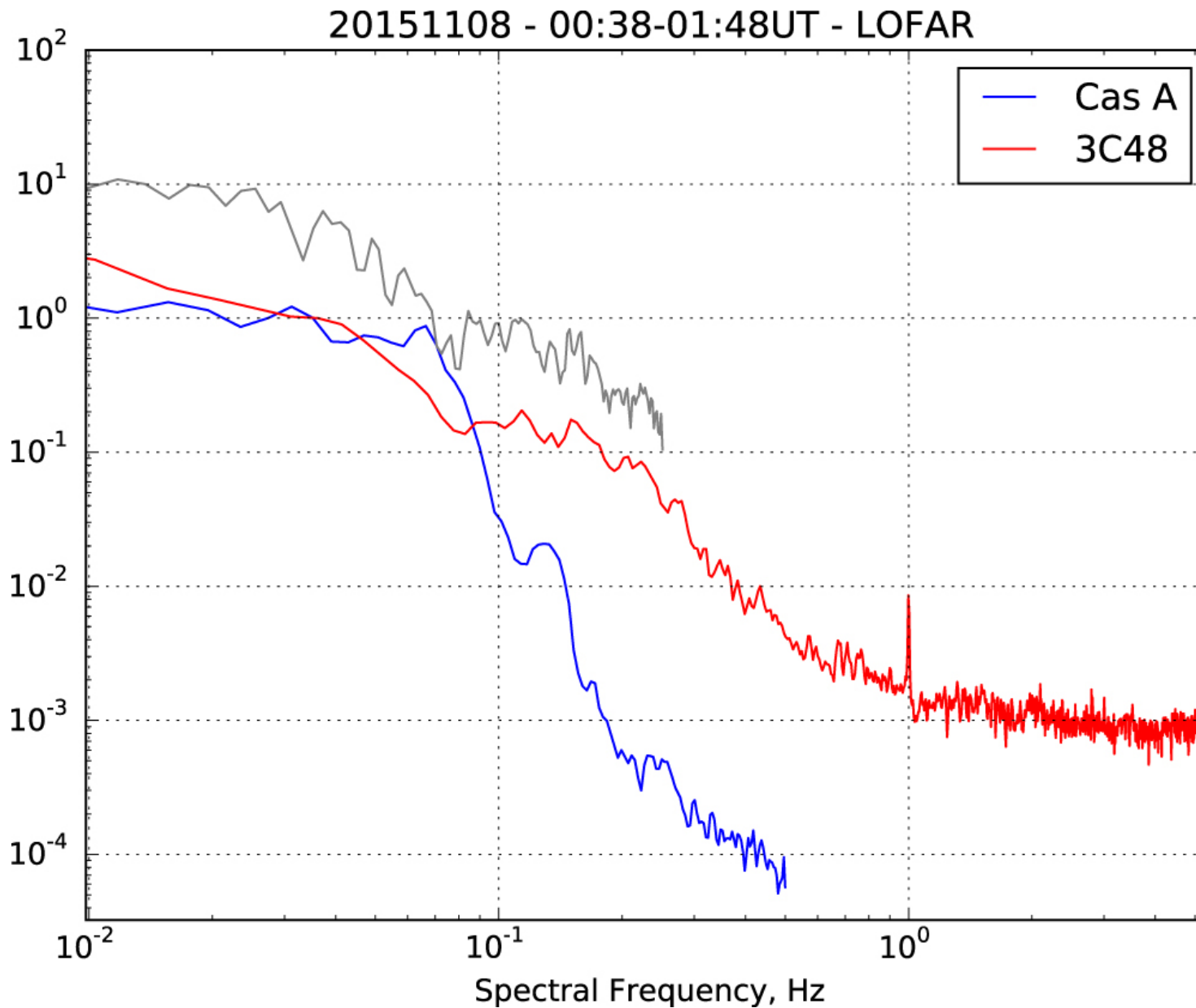
Figure 2. from SEPARATING NIGHTSIDE INTERPLANETARY AND IONOSPHERIC SCINTILLATION WITH LOFAR null 2016 APJL 828 L7 doi:10.3847/2041-8205/828/1/L7 https://dx.doi.org/10.3847/2041-8205/828/1/L7
