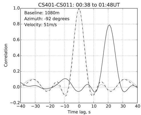
Figure 1. from SEPARATING NIGHTSIDE INTERPLANETARY AND IONOSPHERIC SCINTILLATION WITH LOFAR null 2016 APJL 828 L7 doi:10.3847/2041-8205/828/1/L7 https://dx.doi.org/10.3847/2041-8205/828/1/L7
