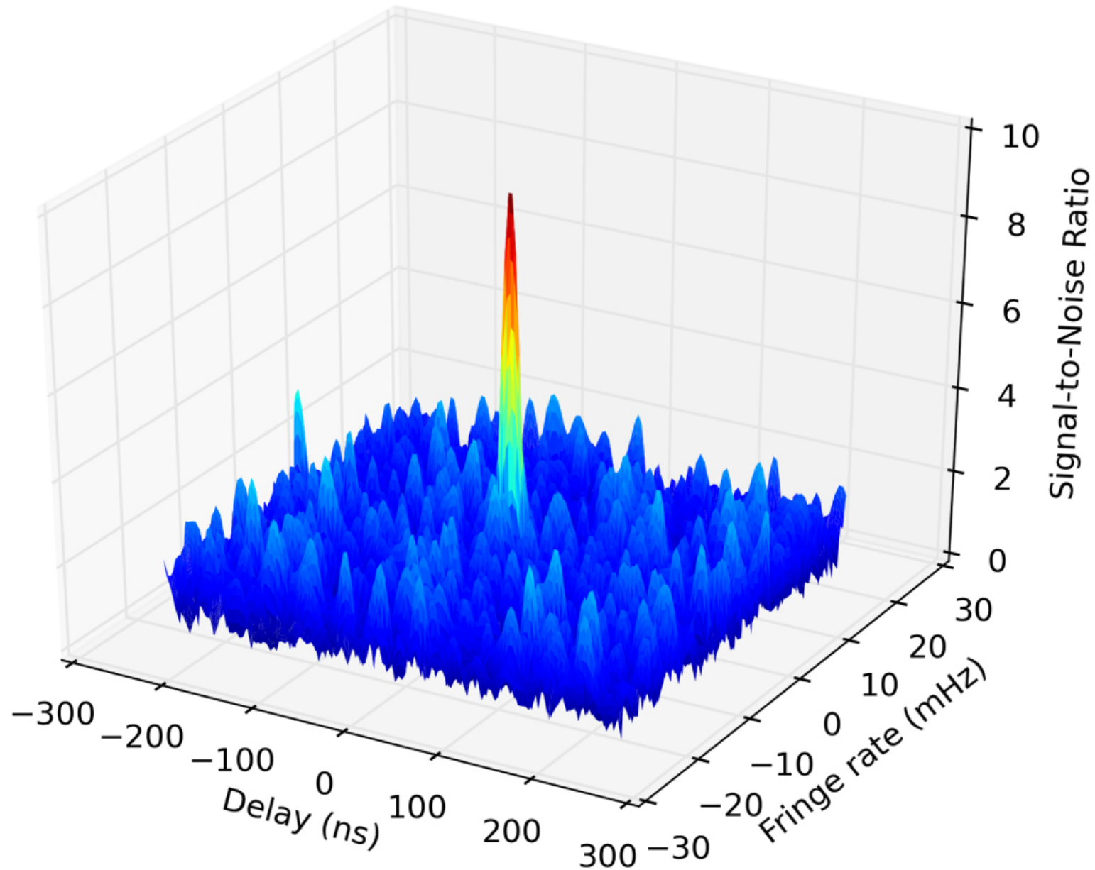
Figure 2. from RADIOASTRON OBSERVATIONS OF THE QUASAR 3C273: A CHALLENGE TO THE BRIGHTNESS TEMPERATURE LIMIT null 2016 APJL 820 L9 doi:10.3847/2041-8205/820/1/L9 https://dx.doi.org/10.3847/2041-8205/820/1/L9 © 2016. The American Astronomical Society. All rights reserved.
