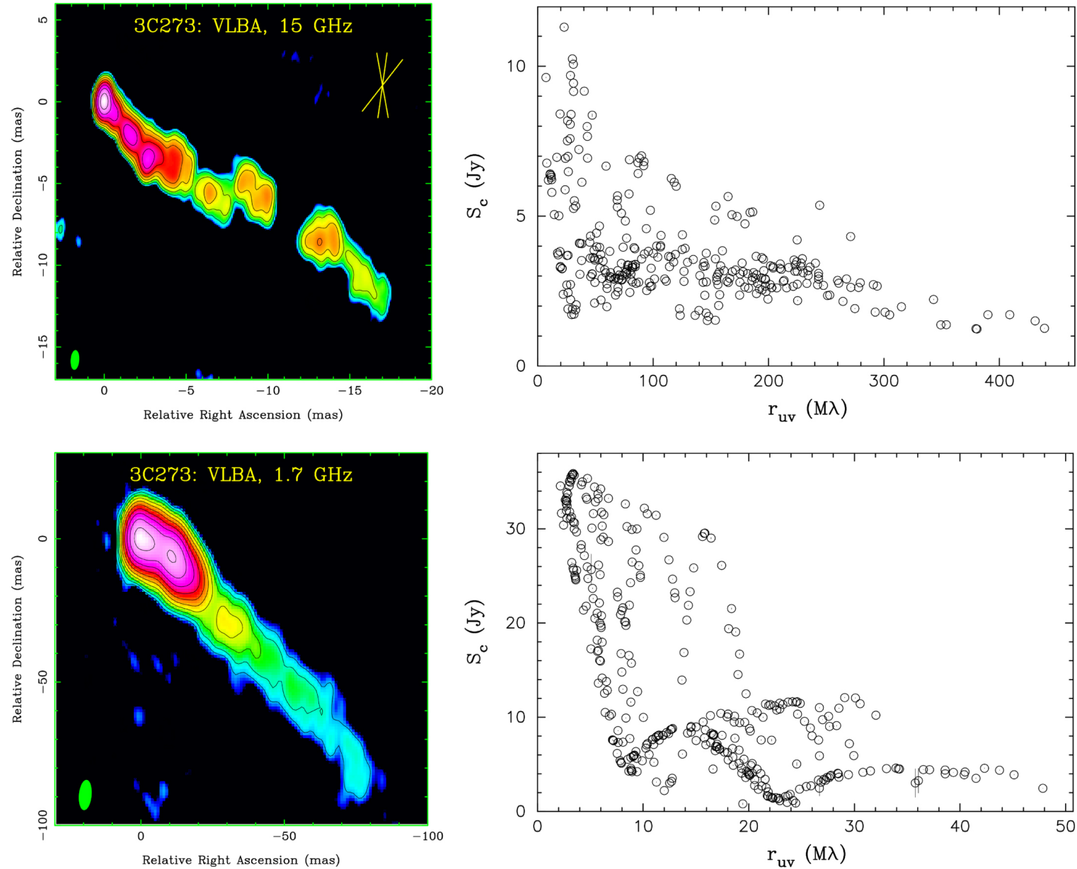
Figure 1. from RADIOASTRON OBSERVATIONS OF THE QUASAR 3C273: A CHALLENGE TO THE BRIGHTNESS TEMPERATURE LIMIT null 2016 APJL 820 L9 doi:10.3847/2041-8205/820/1/L9 https://dx.doi.org/10.3847/2041-8205/820/1/L9 © 2016. The American Astronomical Society. All rights reserved.
