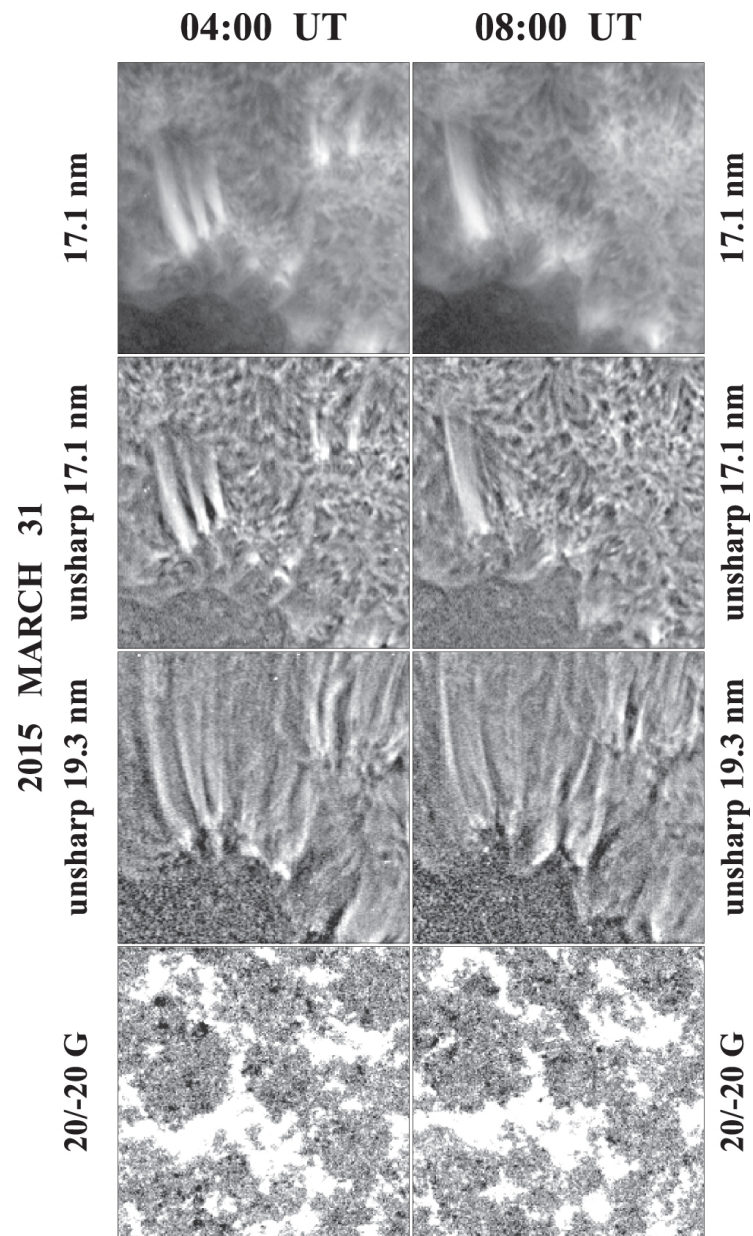
Figure 5. from THE UBIQUITOUS PRESENCE OF LOOPLIKE FINE STRUCTURE INSIDE SOLAR ACTIVE REGIONS null 2016 APJL 820 L13 doi:10.3847/2041-8205/820/1/L13 https://dx.doi.org/10.3847/2041-8205/820/1/L13 Contribution of the Naval Research Laboratory; not subject to copyright in the United States.
