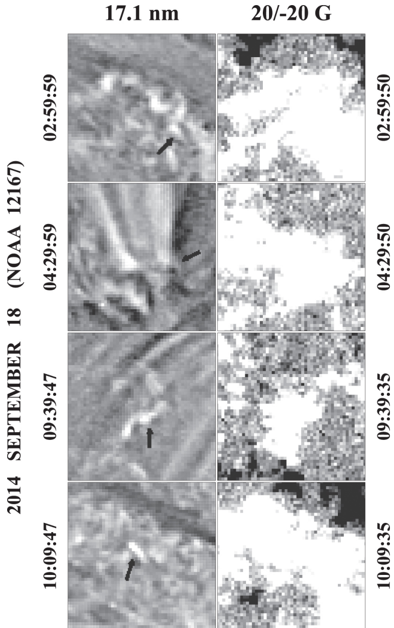
Figure 4. from THE UBIQUITOUS PRESENCE OF LOOPLIKE FINE STRUCTURE INSIDE SOLAR ACTIVE REGIONS null 2016 APJL 820 L13 doi:10.3847/2041-8205/820/1/L13 https://dx.doi.org/10.3847/2041-8205/820/1/L13
