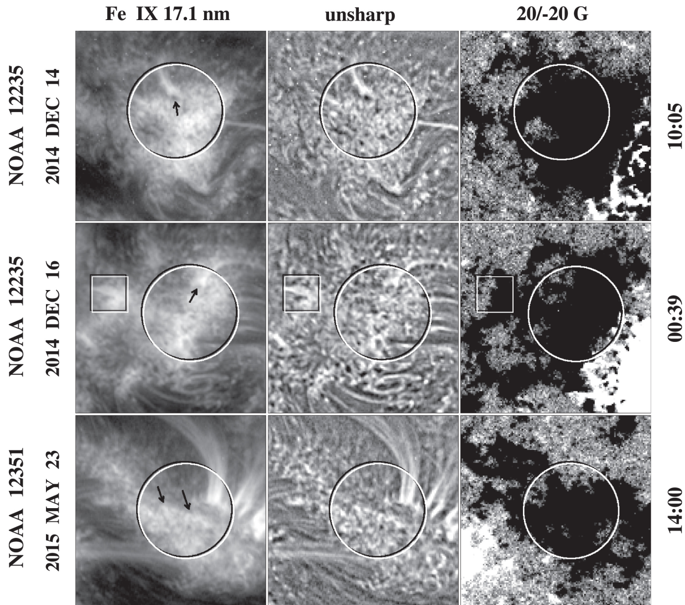
Figure 2. from THE UBIQUITOUS PRESENCE OF LOOPLIKE FINE STRUCTURE INSIDE SOLAR ACTIVE REGIONS null 2016 APJL 820 L13 doi:10.3847/2041-8205/820/1/L13 https://dx.doi.org/10.3847/2041-8205/820/1/L13 Contribution of the Naval Research Laboratory; not subject to copyright in the United States.
