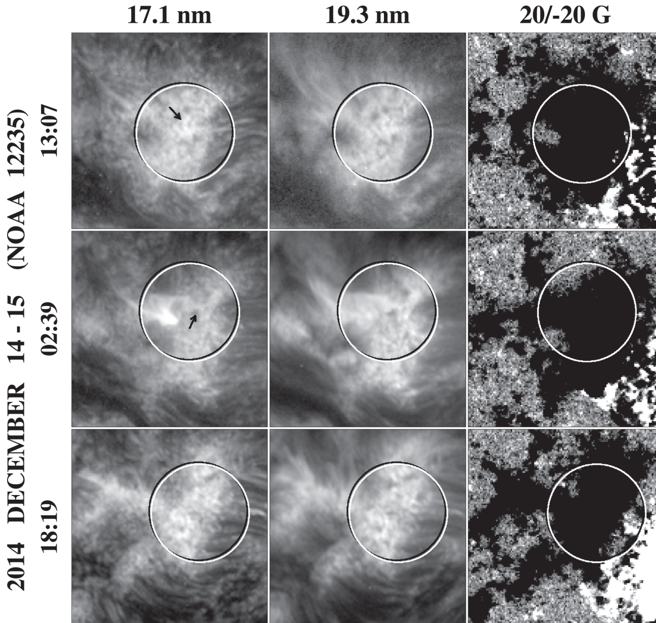
Figure 1. from THE UBIQUITOUS PRESENCE OF LOOPLIKE FINE STRUCTURE INSIDE SOLAR ACTIVE REGIONS null 2016 APJL 820 L13 doi:10.3847/2041-8205/820/1/L13 https://dx.doi.org/10.3847/2041-8205/820/1/L13
