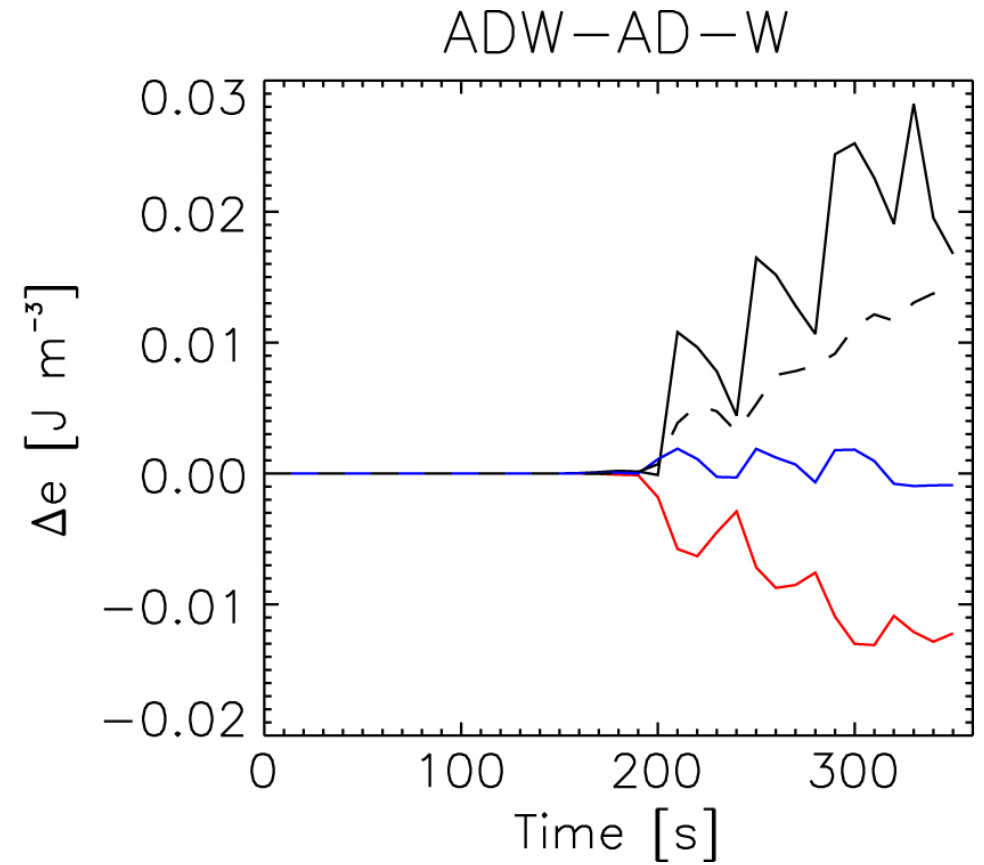
Figure 4. from HEATING OF THE PARTIALLY IONIZED SOLAR CHROMOSPHERE BY WAVES IN MAGNETIC STRUCTURES null 2016 APJL 819 L11 doi:10.3847/2041-8205/819/1/L11 https://dx.doi.org/10.3847/2041-8205/819/1/L11 © 2016. The American Astronomical Society. All rights reserved.
