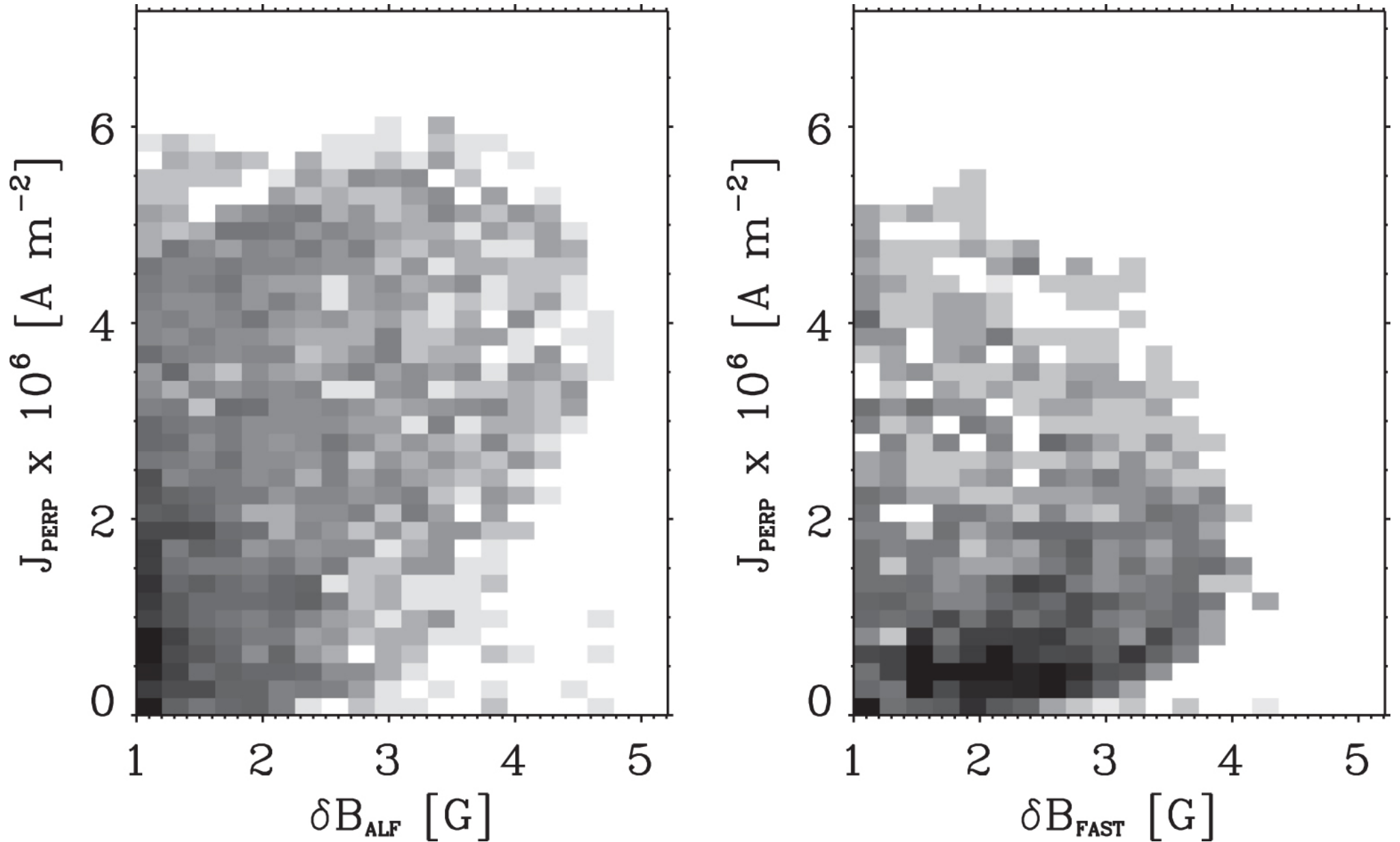
Figure 3. from HEATING OF THE PARTIALLY IONIZED SOLAR CHROMOSPHERE BY WAVES IN MAGNETIC STRUCTURES null 2016 APJL 819 L11 doi:10.3847/2041-8205/819/1/L11 https://dx.doi.org/10.3847/2041-8205/819/1/L11 © 2016. The American Astronomical Society. All rights reserved.
