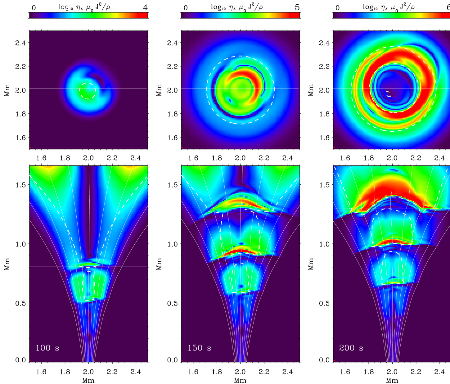
Figure 2. from HEATING OF THE PARTIALLY IONIZED SOLAR CHROMOSPHERE BY WAVES IN MAGNETIC STRUCTURES null 2016 APJL 819 L11 doi:10.3847/2041-8205/819/1/L11 https://dx.doi.org/10.3847/2041-8205/819/1/L11 © 2016. The American Astronomical Society. All rights reserved.
