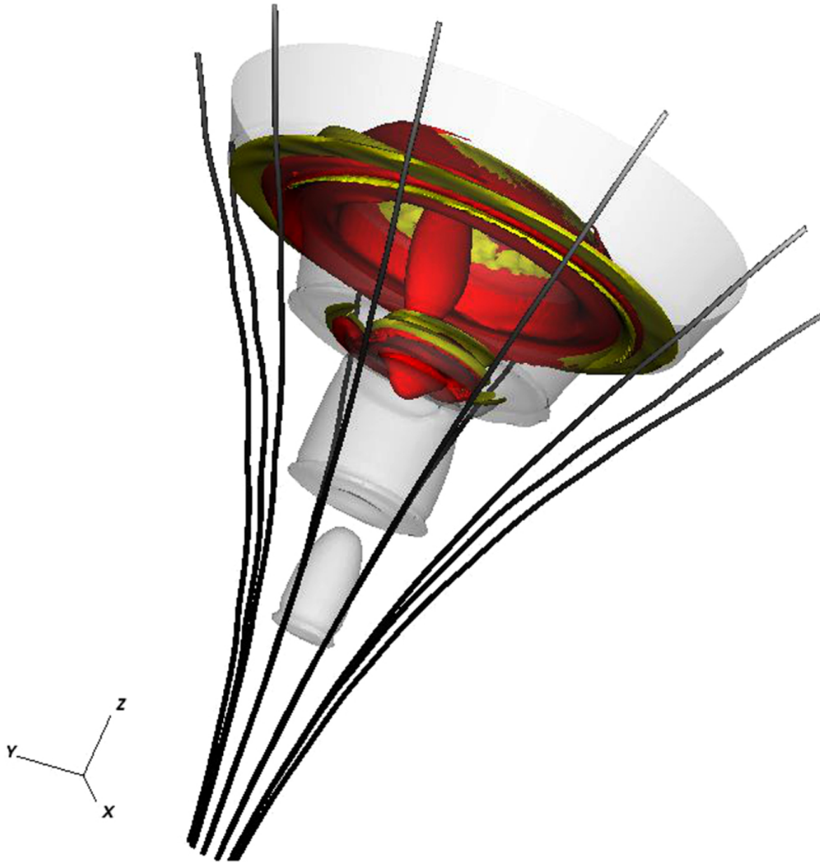
Figure 1. from HEATING OF THE PARTIALLY IONIZED SOLAR CHROMOSPHERE BY WAVES IN MAGNETIC STRUCTURES null 2016 APJL 819 L11 doi:10.3847/2041-8205/819/1/L11 https://dx.doi.org/10.3847/2041-8205/819/1/L11 © 2016. The American Astronomical Society. All rights reserved.
