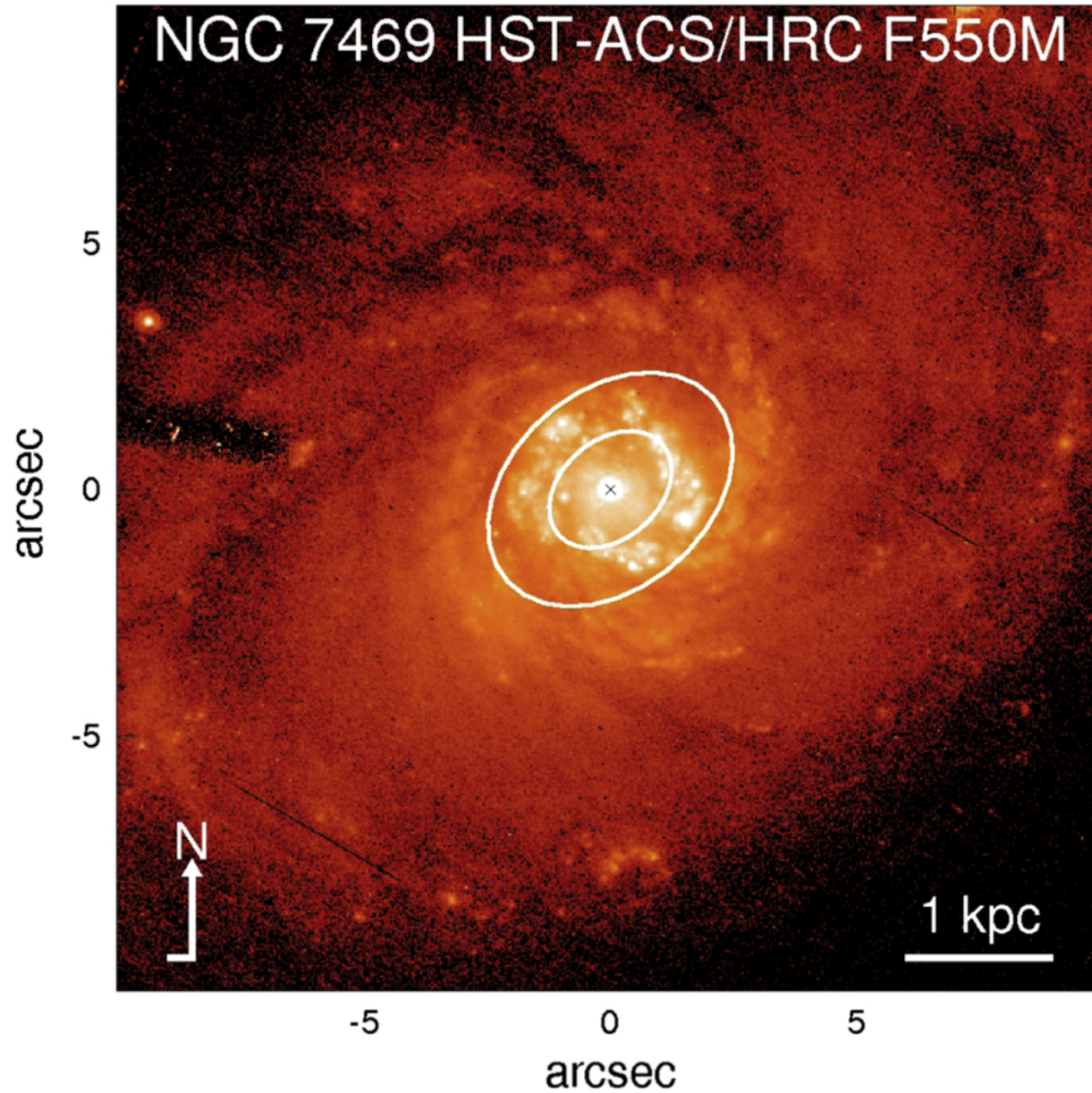
Figure 1. from LOCAL INSTABILITY SIGNATURES IN ALMA OBSERVATIONS OF DENSE GAS IN NGC 7469 null 2015 APJL 806 L34 doi:10.1088/2041-8205/806/2/L34 https://dx.doi.org/10.1088/2041-8205/806/2/L34 © 2015. The American Astronomical Society. All rights reserved.
