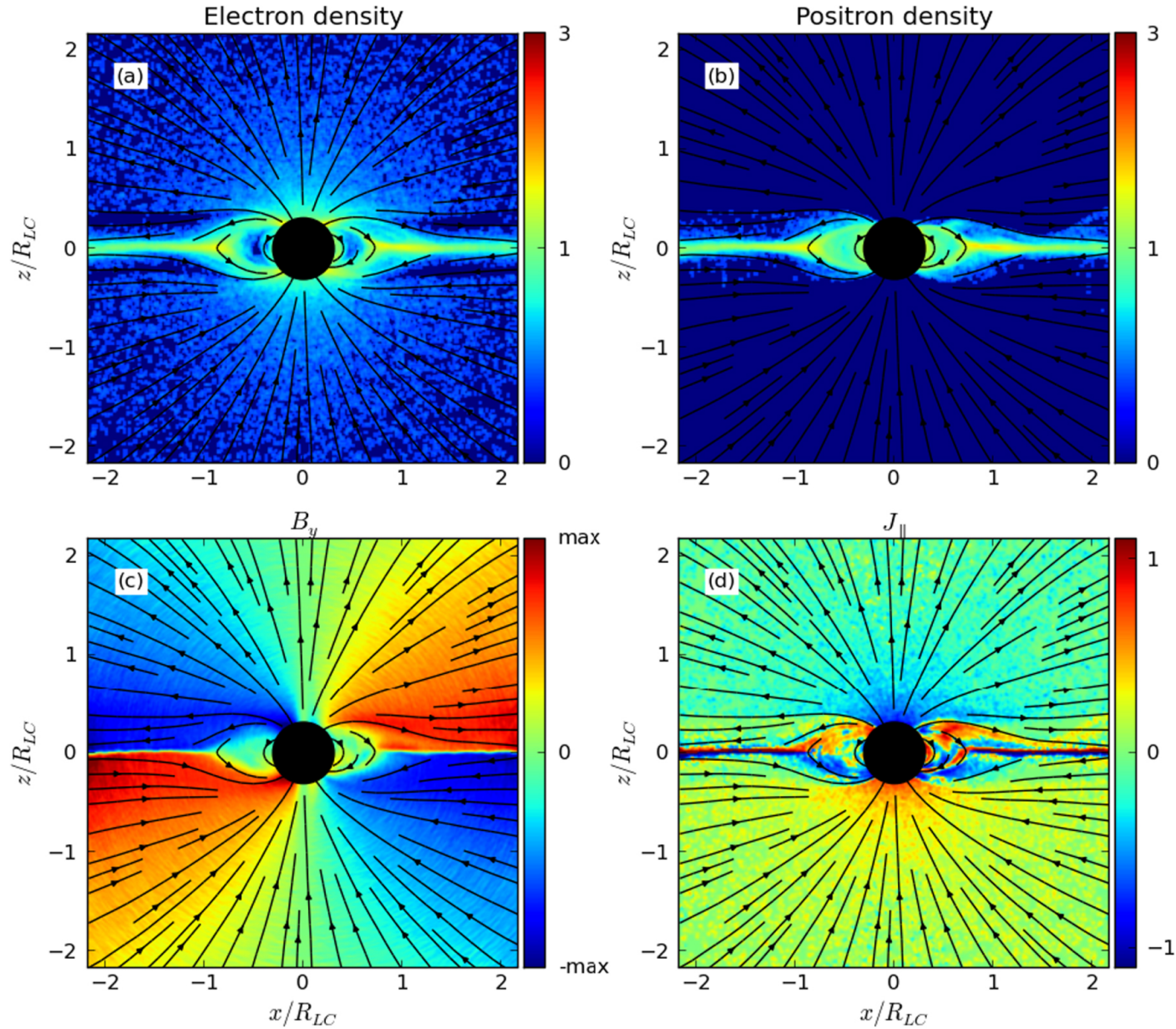
Figure 2. from AB INITIO PULSAR MAGNETOSPHERE: THREE-DIMENSIONAL PARTICLE-IN-CELL SIMULATIONS OF OBLIQUE PULSARS null 2015 APJL 801 L19 doi:10.1088/2041-8205/801/1/L19 https://dx.doi.org/10.1088/2041-8205/801/1/L19 © 2015. The American Astronomical Society. All rights reserved.
