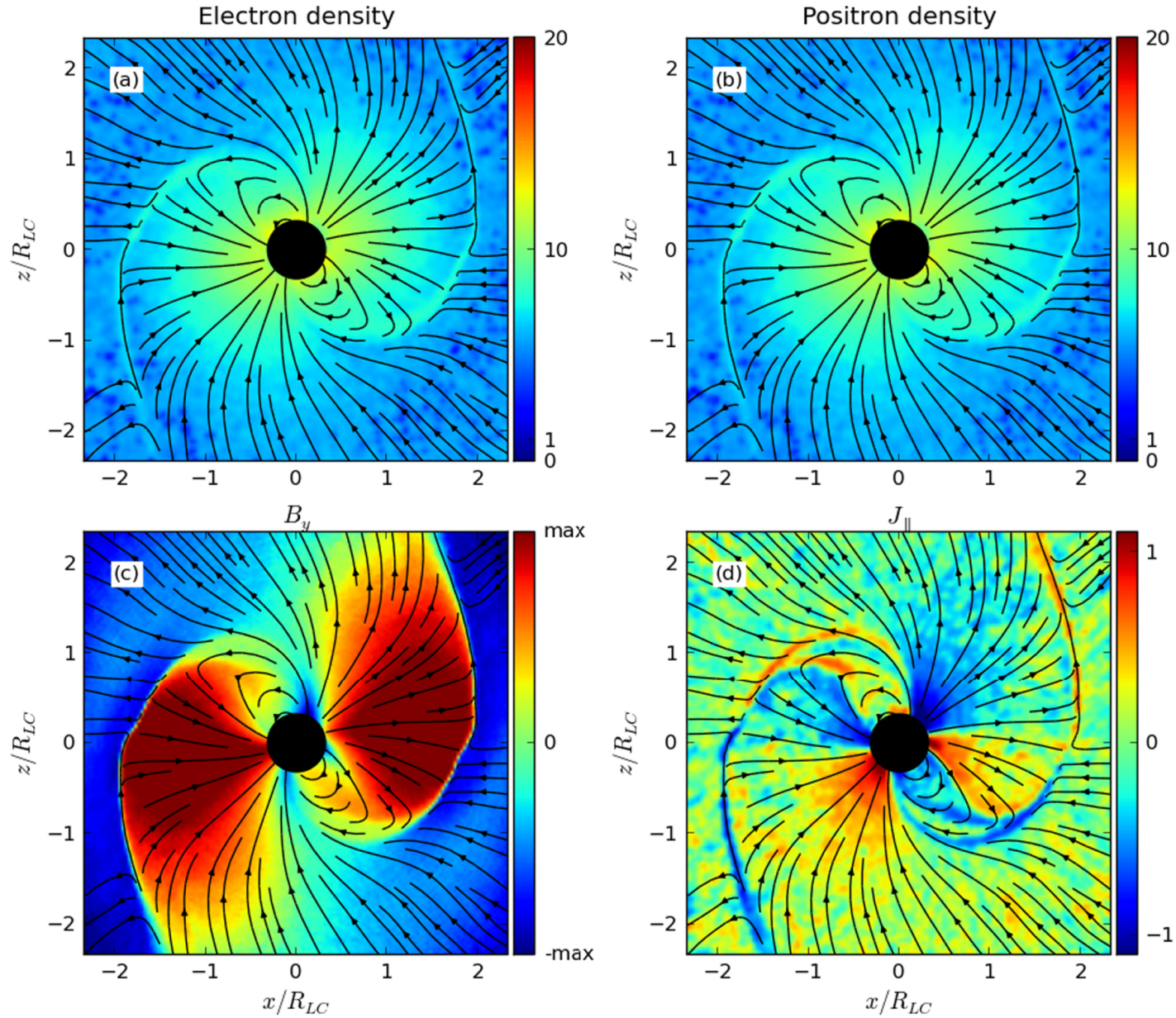
Figure 1. from AB INITIO PULSAR MAGNETOSPHERE: THREE-DIMENSIONAL PARTICLE-IN-CELL SIMULATIONS OF OBLIQUE PULSARS null 2015 APJL 801 L19 doi:10.1088/2041-8205/801/1/L19 https://dx.doi.org/10.1088/2041-8205/801/1/L19 © 2015. The American Astronomical Society. All rights reserved.
