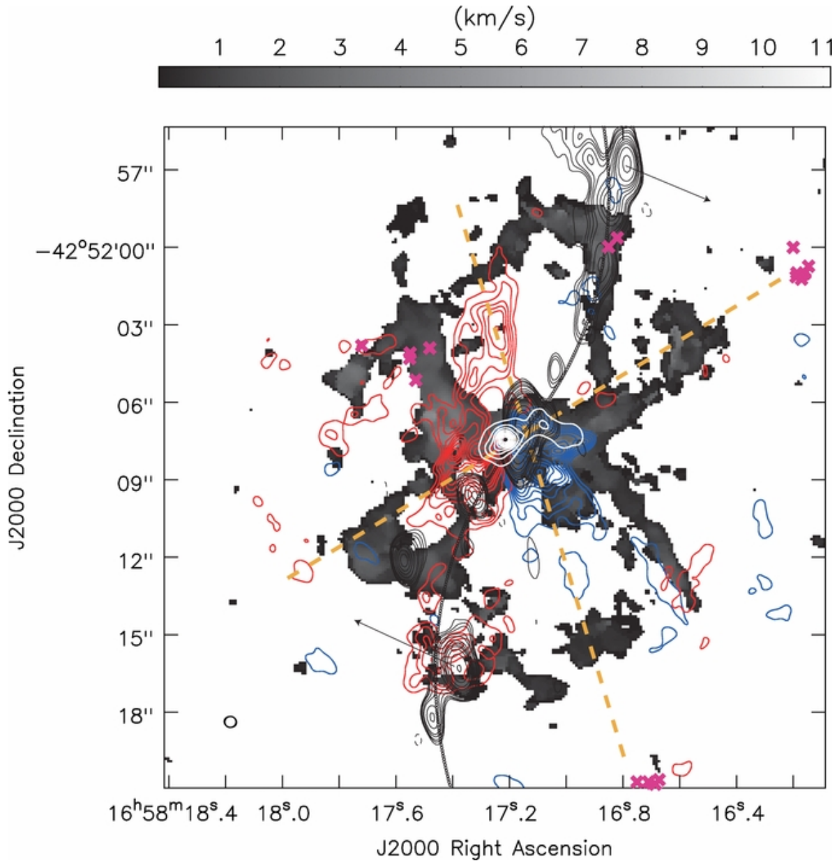
Figure 4. from IRAS 16547–4247: A New Candidate of a Protocluster Unveiled with ALMA Higuchi et al. 2015 ApJL 798 L33 doi:10.1088/2041-8205/798/2/L33 https://dx.doi.org/10.1088/2041-8205/798/2/L33 © 2015. The American Astronomical Society. All rights reserved.
