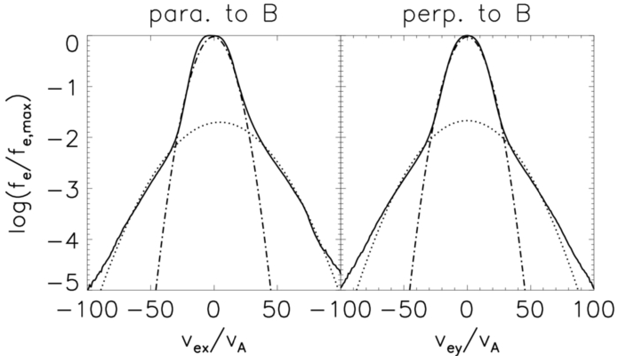
Figure 2. from The Origin of Non-Maxwellian Solar Wind Electron Velocity Distribution Function: Connection to Nanoflares in the Solar Corona Che & Goldstein 2014 ApJL 795 L38 doi:10.1088/2041-8205/795/2/L38 https://dx.doi.org/10.1088/2041-8205/795/2/L38 © 2014. The American Astronomical Society. All rights reserved.
