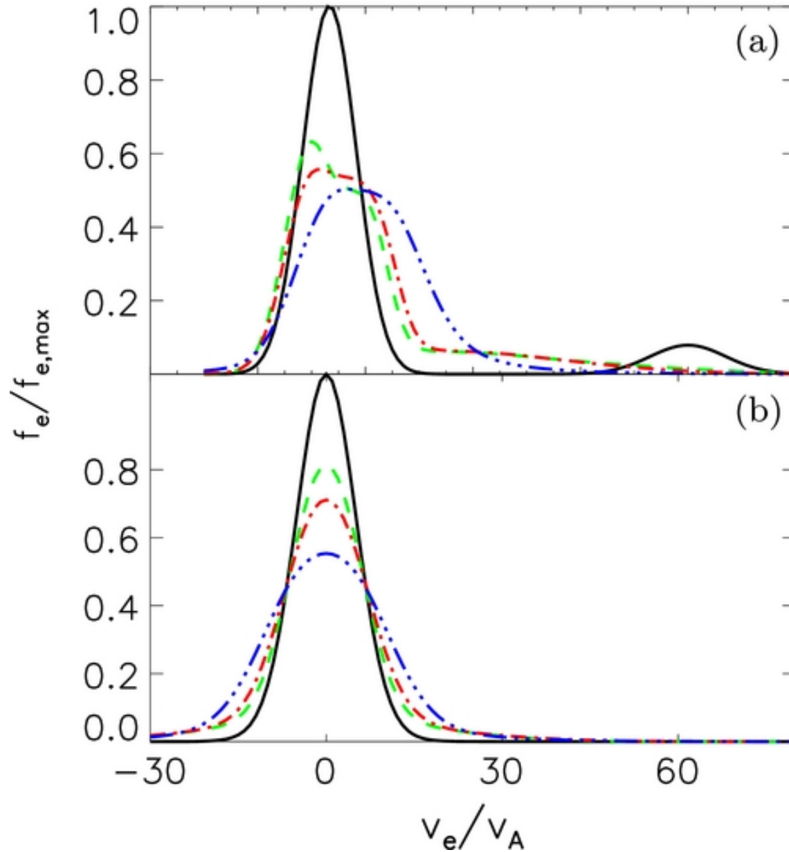
Figure 1. from The Origin of Non-Maxwellian Solar Wind Electron Velocity Distribution Function: Connection to Nanoflares in the Solar Corona Che & Goldstein 2014 ApJL 795 L38 doi:10.1088/2041-8205/795/2/L38 https://dx.doi.org/10.1088/2041-8205/795/2/L38 © 2014. The American Astronomical Society. All rights reserved.
