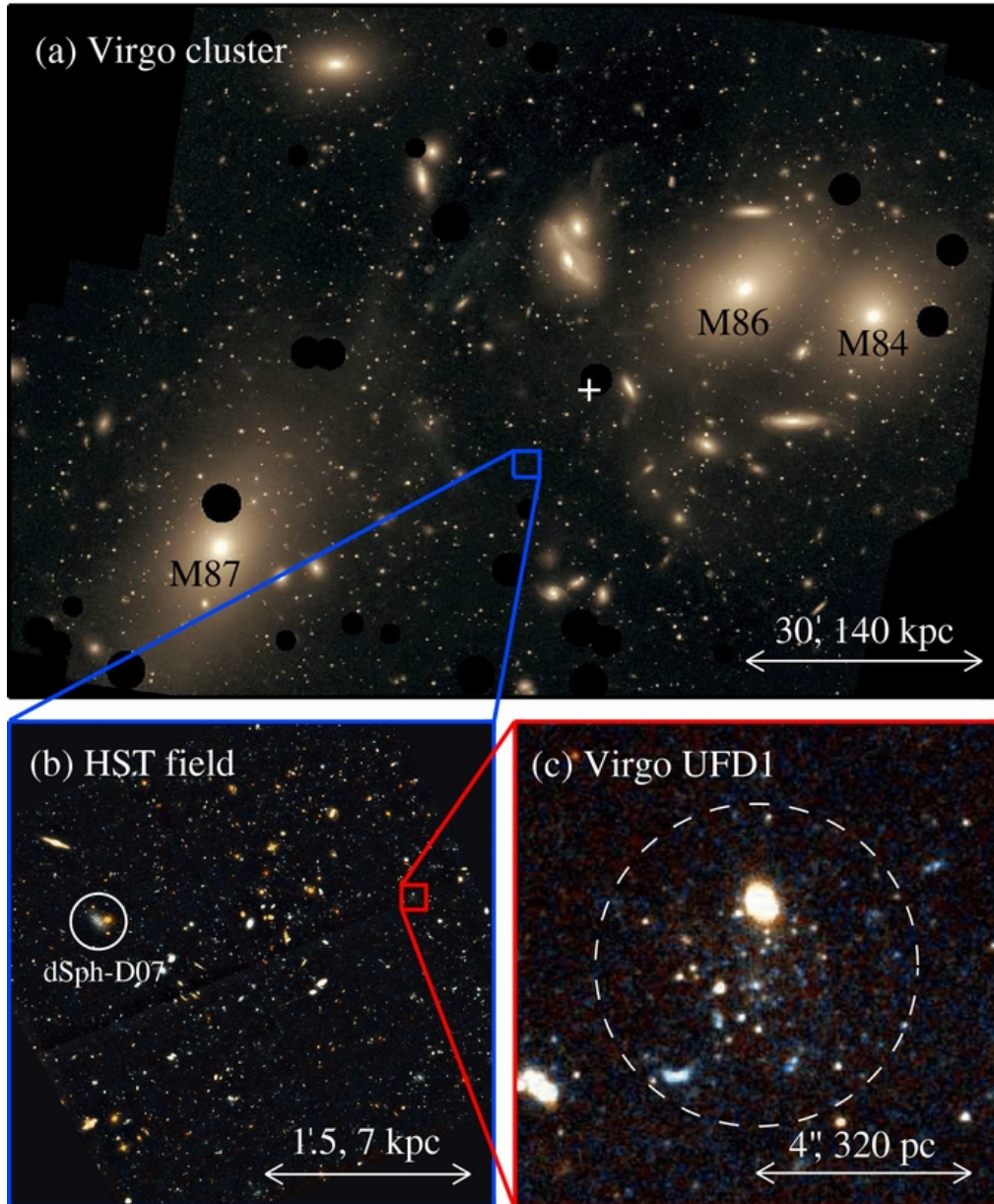
Figure 1. from Discovery of an Ultra-faint Dwarf Galaxy in the Intracluster Field of the Virgo Center: A Fossil of the First Galaxies? Jang & Lee 2014 ApJL 795 L6 doi:10.1088/2041-8205/795/1/L6 https://dx.doi.org/10.1088/2041-8205/795/1/L6 © 2014. The American Astronomical Society. All rights reserved.
