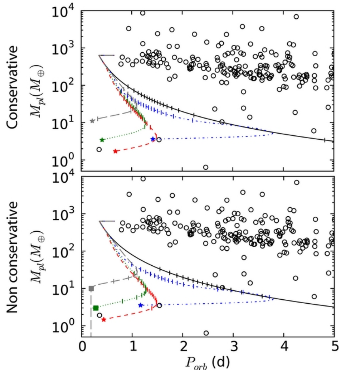
Figure 4. from From Hot Jupiters to Super-Earths via Roche Lobe Overflow Valsecchi, Rasio, & Steffen 2014 ApJL 793 L3 doi:10.1088/2041-8205/793/1/L3 https://dx.doi.org/10.1088/2041-8205/793/1/L3 © 2014. The American Astronomical Society. All rights reserved.
