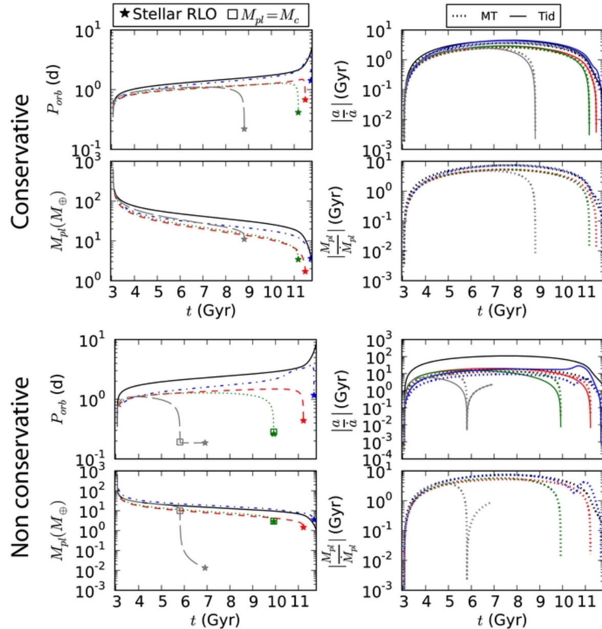
Figure 3. from From Hot Jupiters to Super-Earths via Roche Lobe Overflow Valsecchi, Rasio, & Steffen 2014 ApJL 793 L3 doi:10.1088/2041-8205/793/1/L3 https://dx.doi.org/10.1088/2041-8205/793/1/L3
