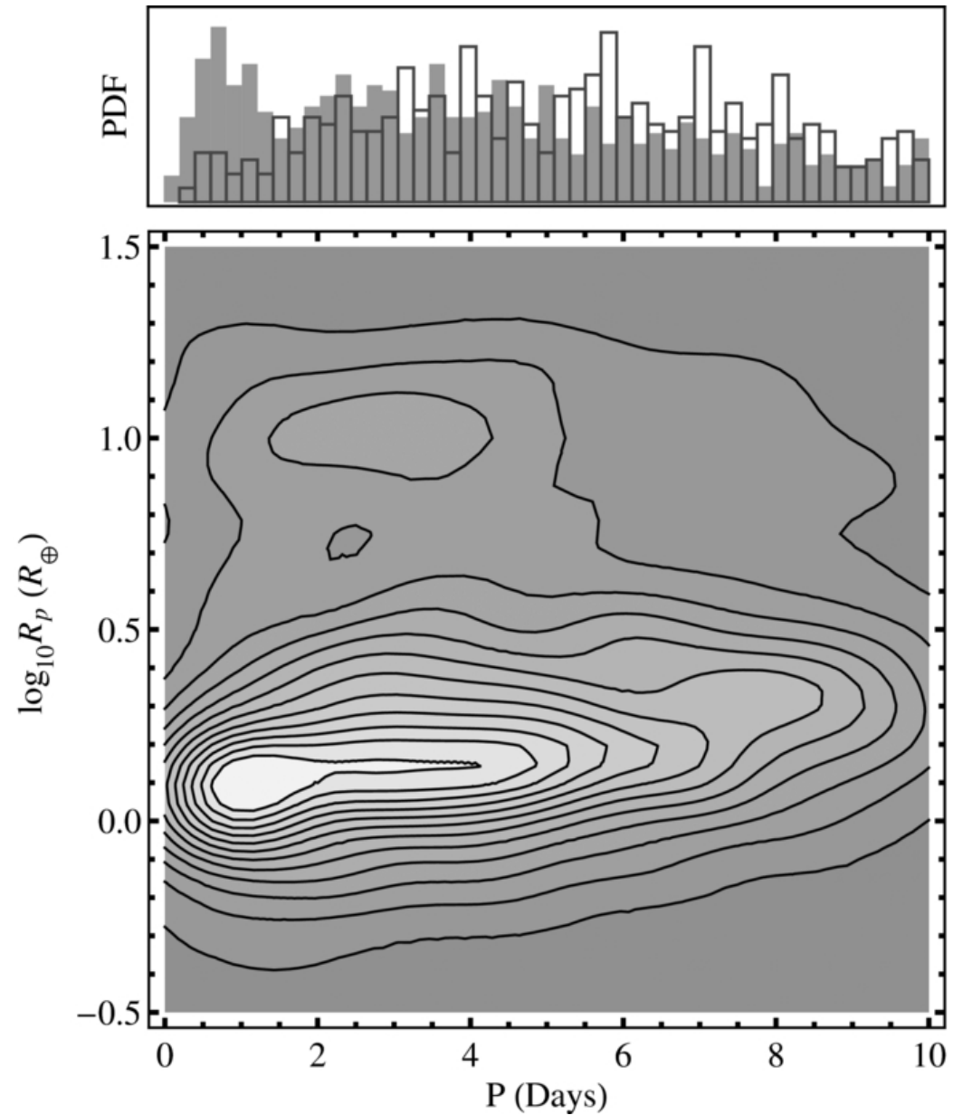
Figure 1. from From Hot Jupiters to Super-Earths via Roche Lobe Overflow Valsecchi, Rasio, & Steffen 2014 ApJL 793 L3 doi:10.1088/2041-8205/793/1/L3 https://dx.doi.org/10.1088/2041-8205/793/1/L3 © 2014. The American Astronomical Society. All rights reserved.
