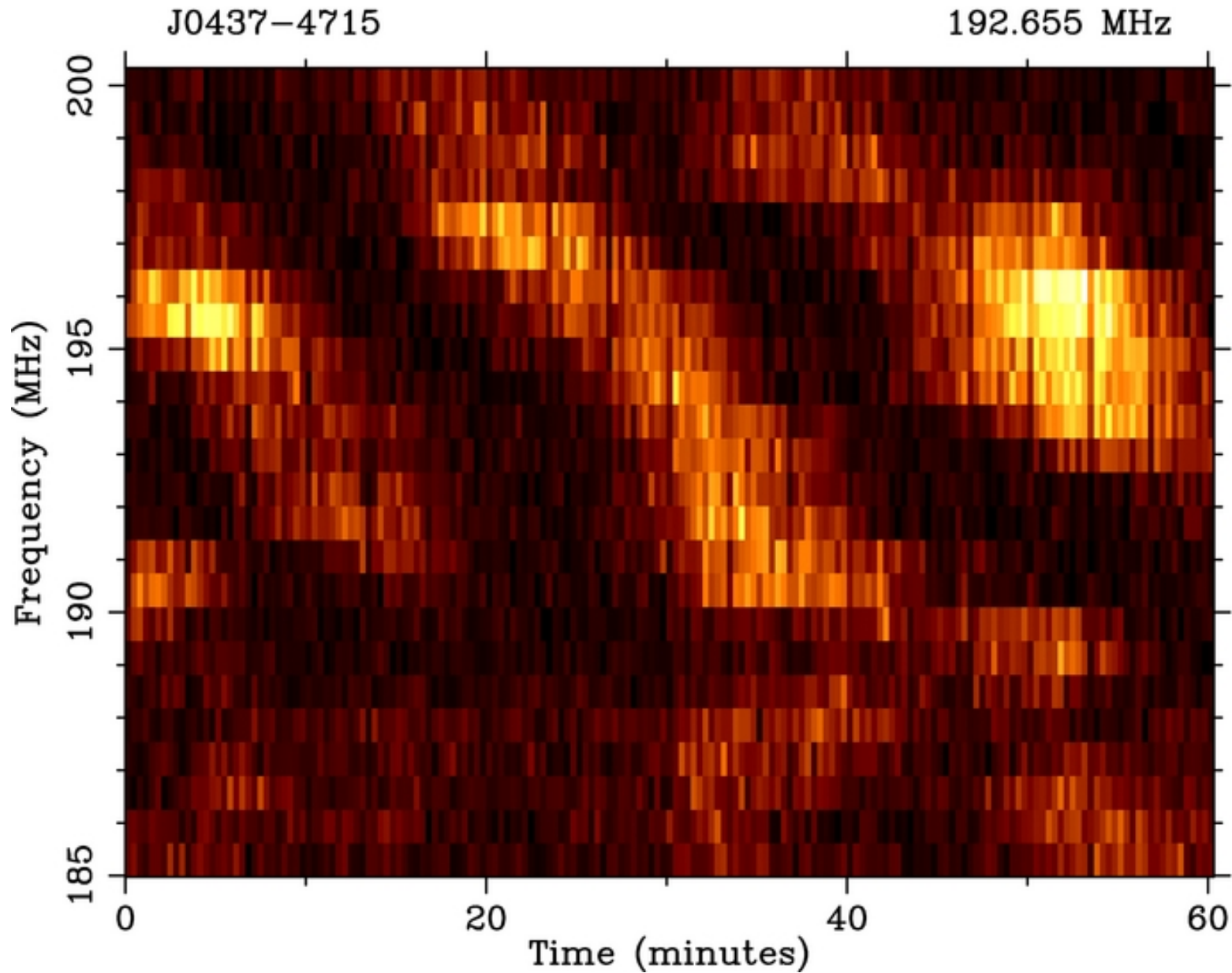
Figure 2. from The Low-frequency Characteristics of PSR J0437–4715 Observed with the Murchison Wide-field Array Bhat et al. 2014 ApJL 791 L32 doi:10.1088/2041-8205/791/2/L32 https://dx.doi.org/10.1088/2041-8205/791/2/L32 © 2014. The American Astronomical Society. All rights reserved.
