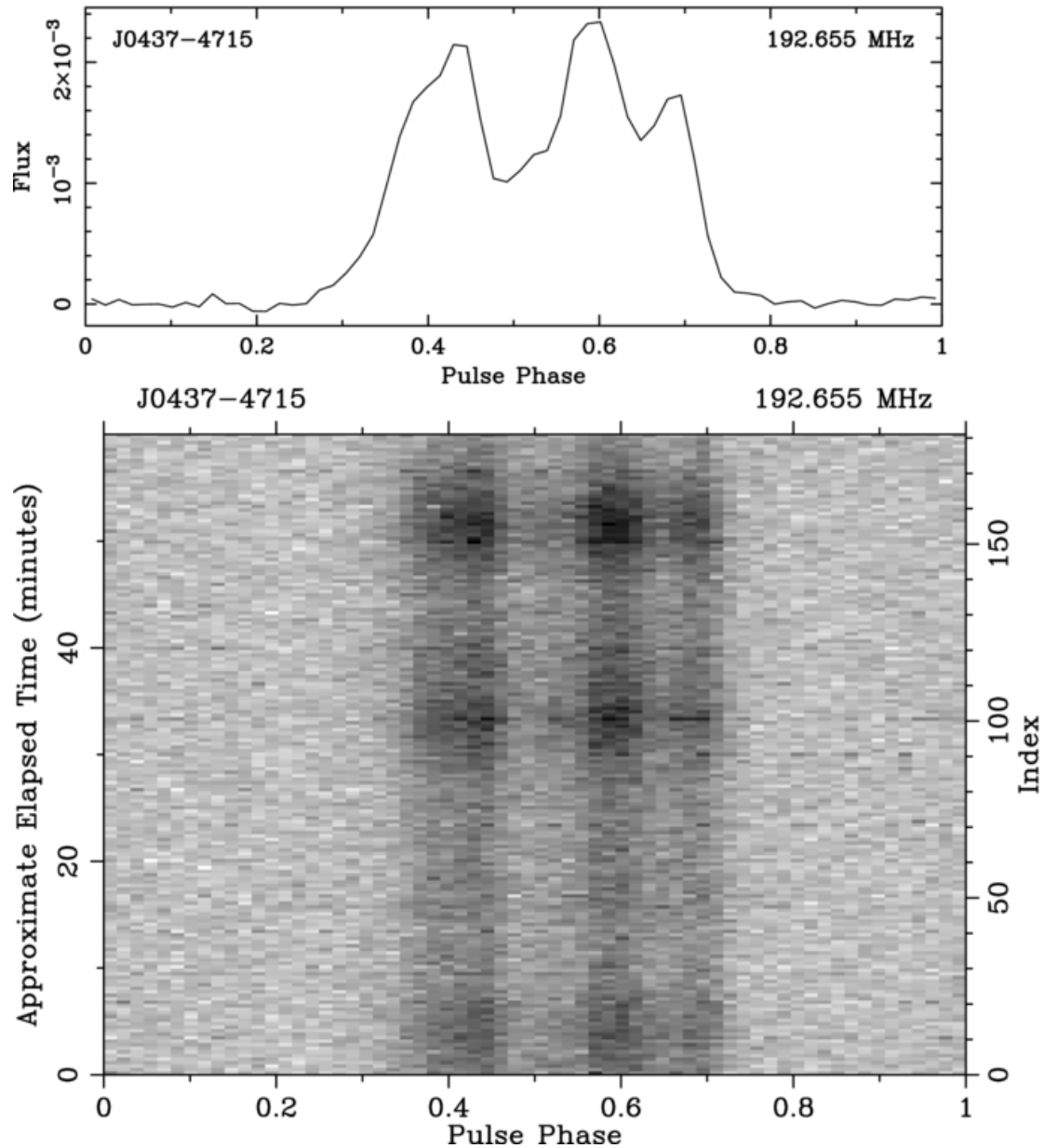
Figure 1. from The Low-frequency Characteristics of PSR J0437–4715 Observed with the Murchison Wide-field Array Bhat et al. 2014 ApJL 791 L32 doi:10.1088/2041-8205/791/2/L32 https://dx.doi.org/10.1088/2041-8205/791/2/L32 © 2014. The American Astronomical Society. All rights reserved.
