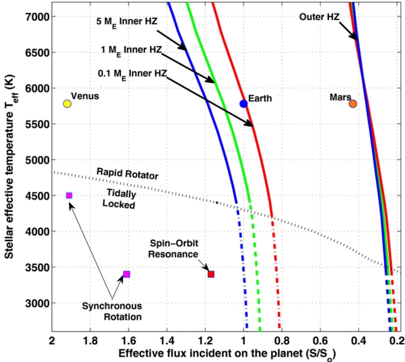
Figure 3. from Habitable Zones around Main-sequence Stars: Dependence on Planetary Mass Kopparapu et al. 2014 ApJL 787 L29 doi:10.1088/2041-8205/787/2/L29 https://dx.doi.org/10.1088/2041-8205/787/2/L29 © 2014. The American Astronomical Society. All rights reserved.
