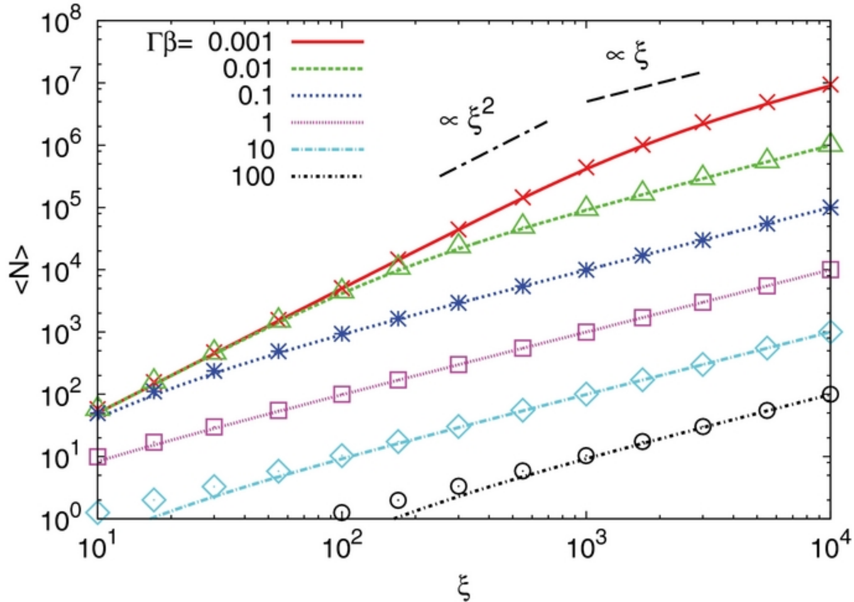
Figure 2. from Random Walks and Effective Optical Depth in Relativistic Flow Shibata, Tominaga, & Tanaka 2014 ApJL 787 L4 doi:10.1088/2041-8205/787/1/L4 https://dx.doi.org/10.1088/2041-8205/787/1/L4 © 2014. The American Astronomical Society. All rights reserved.
