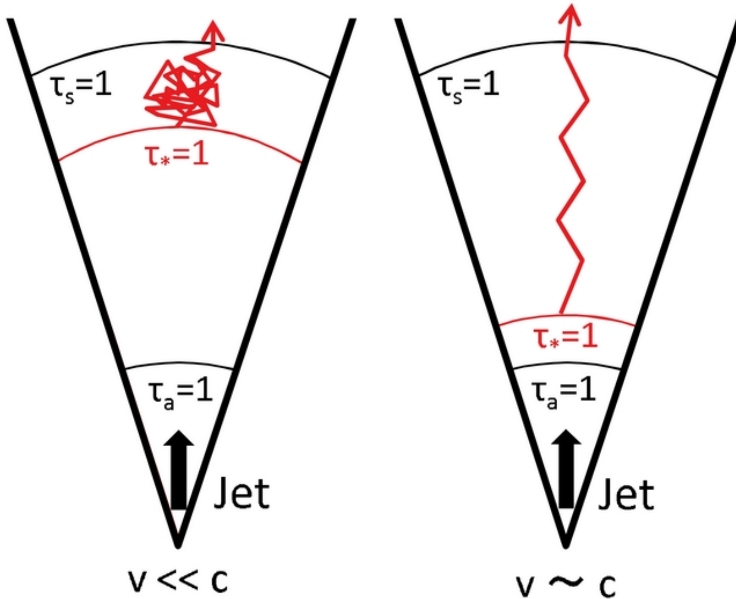
Figure 1. from Random Walks and Effective Optical Depth in Relativistic Flow Shibata, Tominaga, & Tanaka 2014 ApJL 787 L4 doi:10.1088/2041-8205/787/1/L4 https://dx.doi.org/10.1088/2041-8205/787/1/L4 © 2014. The American Astronomical Society. All rights reserved.
