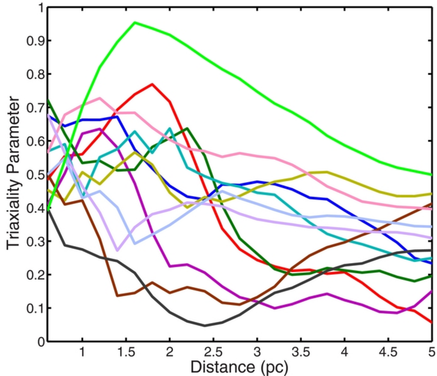
Figure 3. from Age and Mass Segregation of Multiple Stellar Populations in Galactic Nuclei and their Observational Signatures Perets & Mastrobuono-Battisti 2014 ApJL 784 L44 doi:10.1088/2041-8205/784/2/L44 https://dx.doi.org/10.1088/2041-8205/784/2/L44 © 2014. The American Astronomical Society. All rights reserved.
