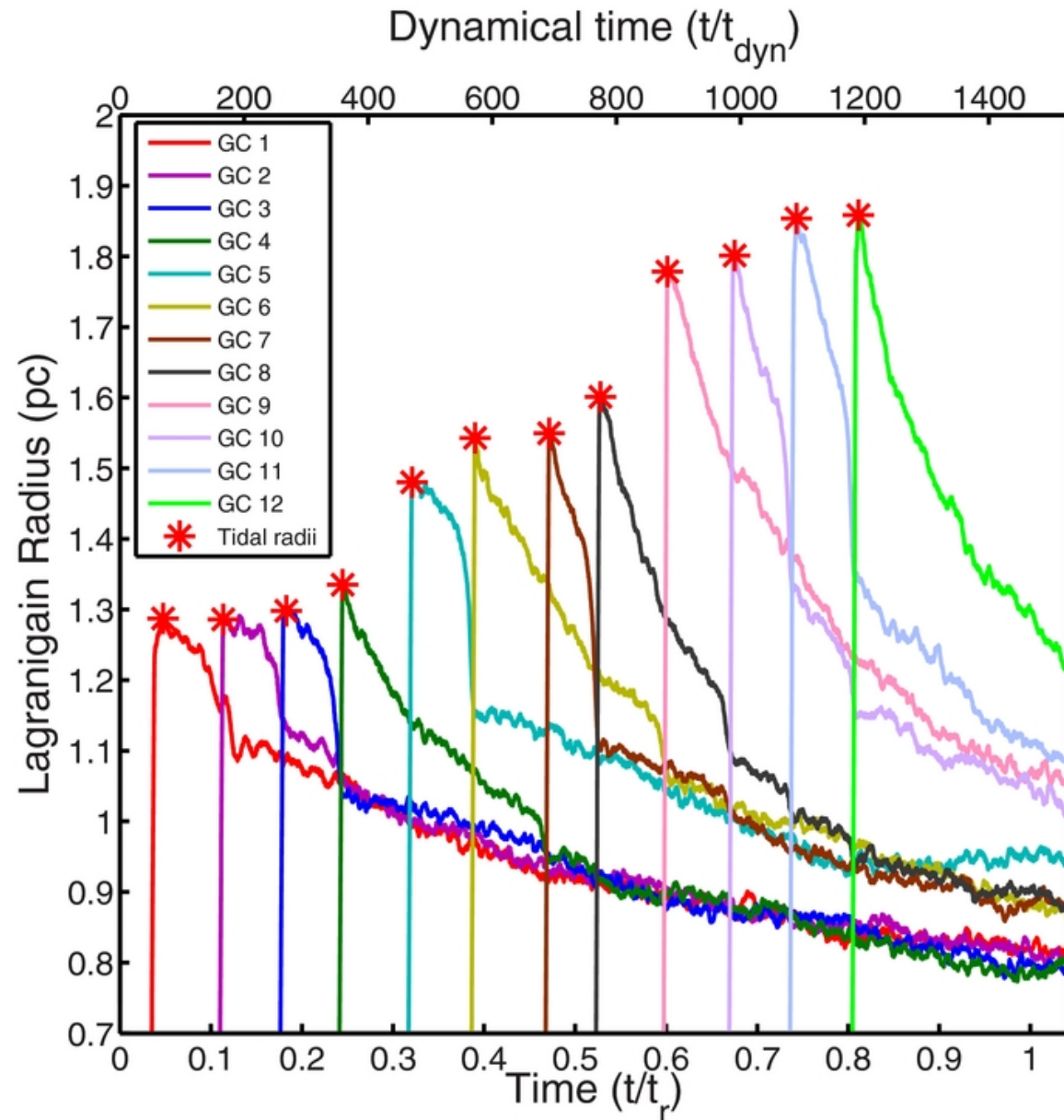
Figure 2. from Age and Mass Segregation of Multiple Stellar Populations in Galactic Nuclei and their Observational Signatures Perets & Mastrobuono-Battisti 2014 ApJL 784 L44 doi:10.1088/2041-8205/784/2/L44 https://dx.doi.org/10.1088/2041-8205/784/2/L44 © 2014. The American Astronomical Society. All rights reserved.
