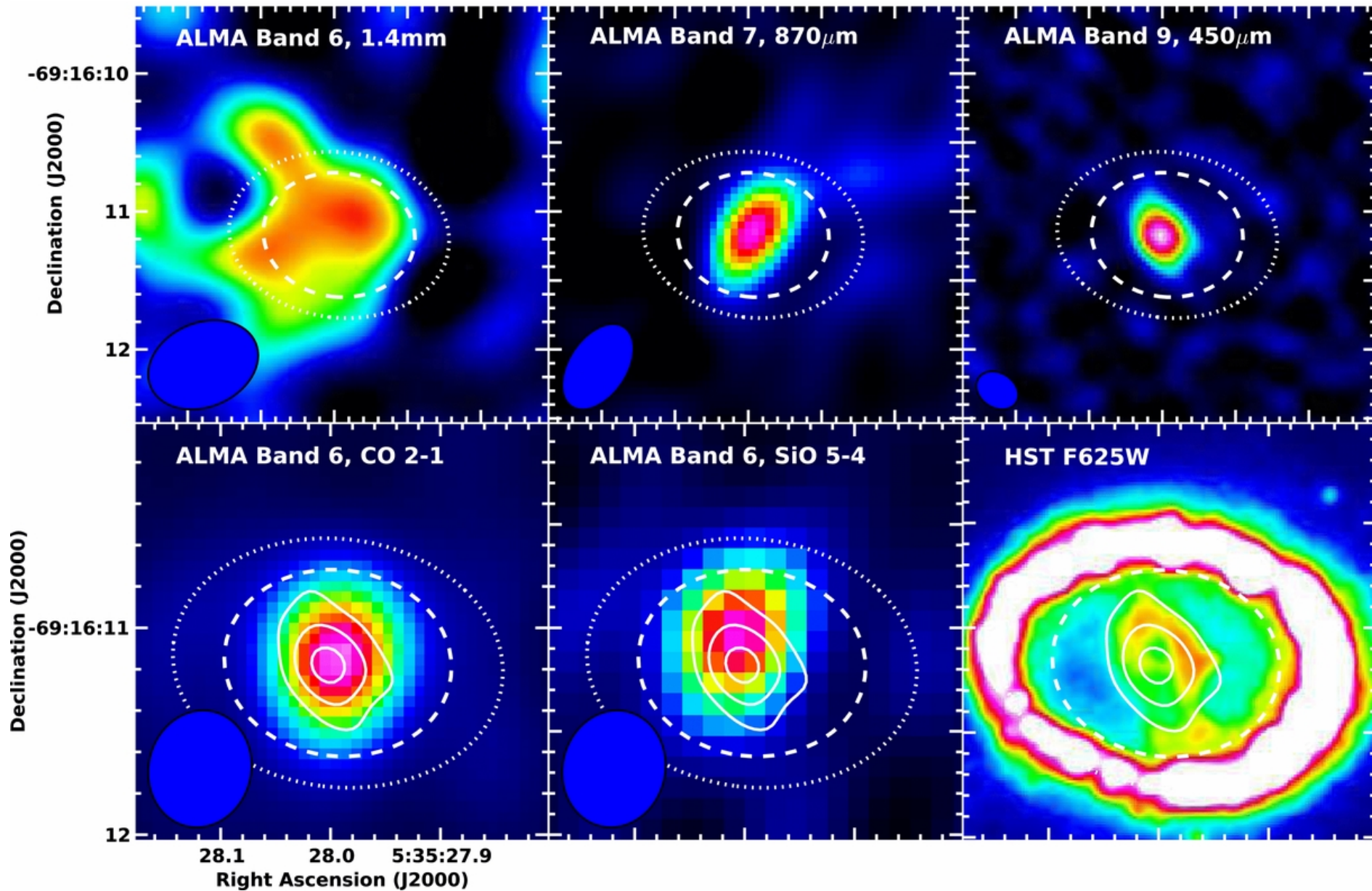
Figure 4. from Dust Production and Particle Acceleration in Supernova 1987A Revealed with ALMA Indebetouw et al. 2014 ApJL 782 L2 doi:10.1088/2041-8205/782/1/L2 https://dx.doi.org/10.1088/2041-8205/782/1/L2 © 2014. The American Astronomical Society. All rights reserved.
