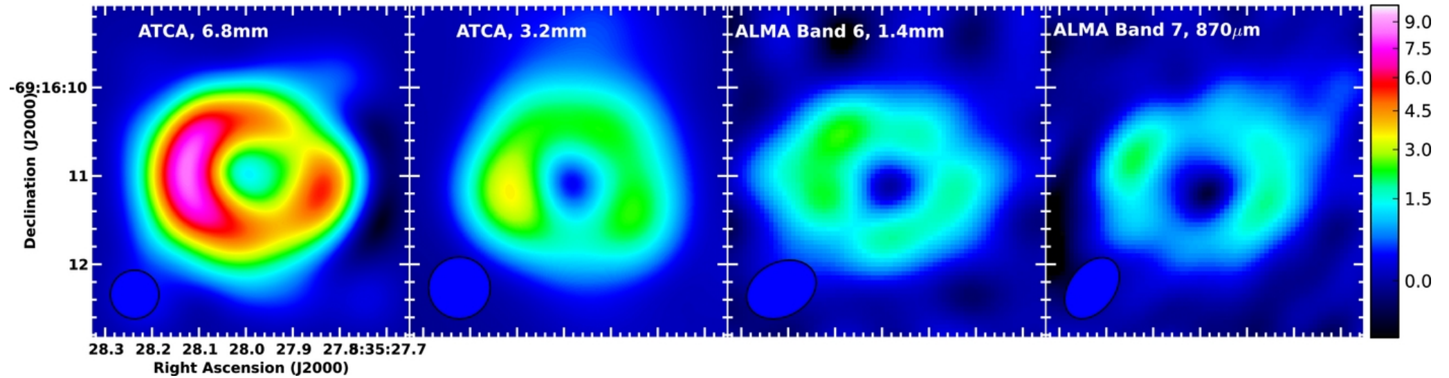
Figure 2. from Dust Production and Particle Acceleration in Supernova 1987A Revealed with ALMA Indebetouw et al. 2014 ApJL 782 L2 doi:10.1088/2041-8205/782/1/L2 https://dx.doi.org/10.1088/2041-8205/782/1/L2 © 2014. The American Astronomical Society. All rights reserved.
