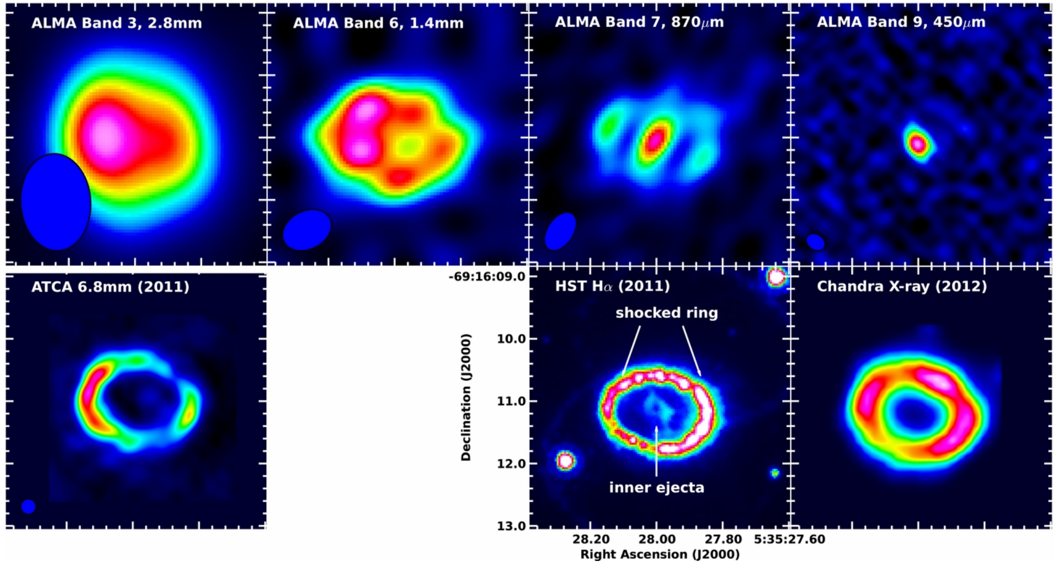
Figure 1. from Dust Production and Particle Acceleration in Supernova 1987A Revealed with ALMA Indebetouw et al. 2014 ApJL 782 L2 doi:10.1088/2041-8205/782/1/L2 https://dx.doi.org/10.1088/2041-8205/782/1/L2 © 2014. The American Astronomical Society. All rights reserved.
