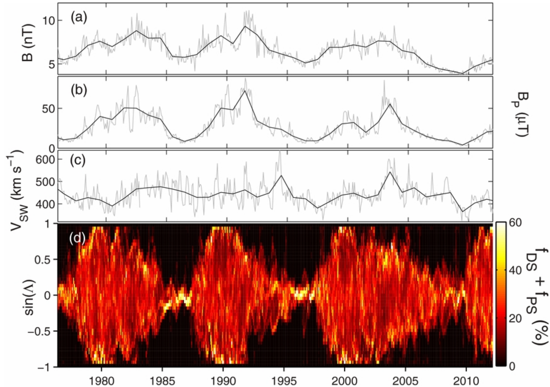
Figure 4. from Implications of the Recent Low Solar Minimum for the Solar Wind during the Maunder Minimum Lockwood & Owens 2014 ApJL 781 L7 doi:10.1088/2041-8205/781/1/L7 https://dx.doi.org/10.1088/2041-8205/781/1/L7 © 2014. The American Astronomical Society. All rights reserved.
