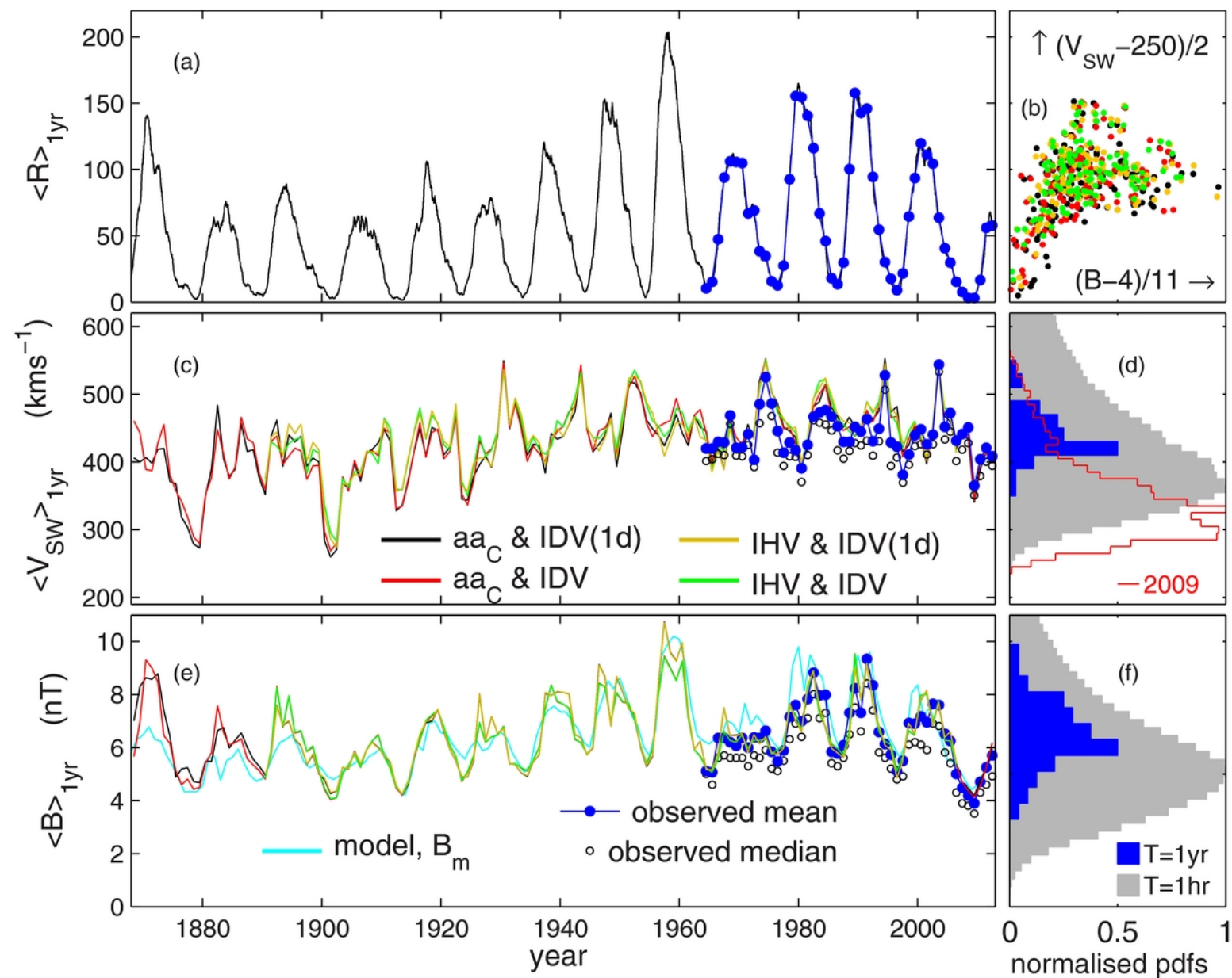
Figure 2. from Implications of the Recent Low Solar Minimum for the Solar Wind during the Maunder Minimum Lockwood & Owens 2014 ApJL 781 L7 doi:10.1088/2041-8205/781/1/L7 https://dx.doi.org/10.1088/2041-8205/781/1/L7 © 2014. The American Astronomical Society. All rights reserved.
