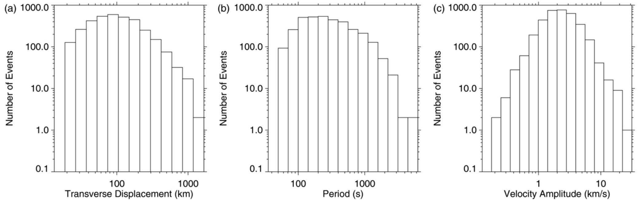
Figure 4. from A Statistical Study of Transverse Oscillations in a Quiescent Prominence Hillier, Morton, & Erdélyi 2013 ApJL 779 L16 doi:10.1088/2041-8205/779/2/L16 https://dx.doi.org/10.1088/2041-8205/779/2/L16 © 2013. The American Astronomical Society. All rights reserved.
