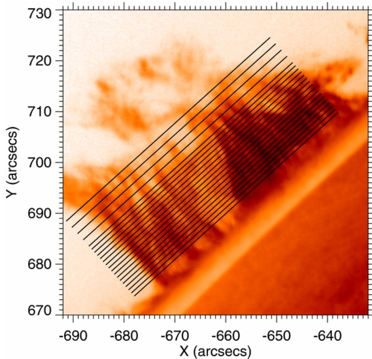
Figure 1. from A Statistical Study of Transverse Oscillations in a Quiescent Prominence Hillier, Morton, & Erdélyi 2013 ApJL 779 L16 doi:10.1088/2041-8205/779/2/L16 https://dx.doi.org/10.1088/2041-8205/779/2/L16 © 2013. The American Astronomical Society. All rights reserved.
