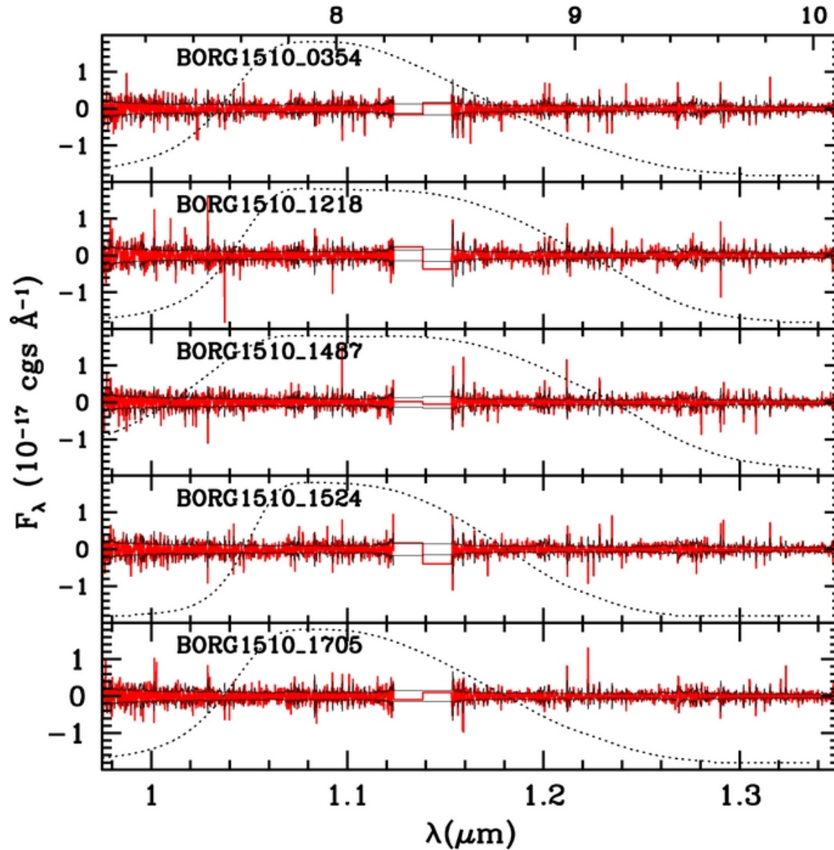
Figure 2. from The Changing Ly Optical Depth in the Range 6 < z < 9 from the MOSFIRE Spectroscopy of Y-dropouts Treu et al. 2013 ApJL 775 L29 doi:10.1088/2041-8205/775/1/L29 https://dx.doi.org/10.1088/2041-8205/775/1/L29 © 2013. The American Astronomical Society. All rights reserved.
