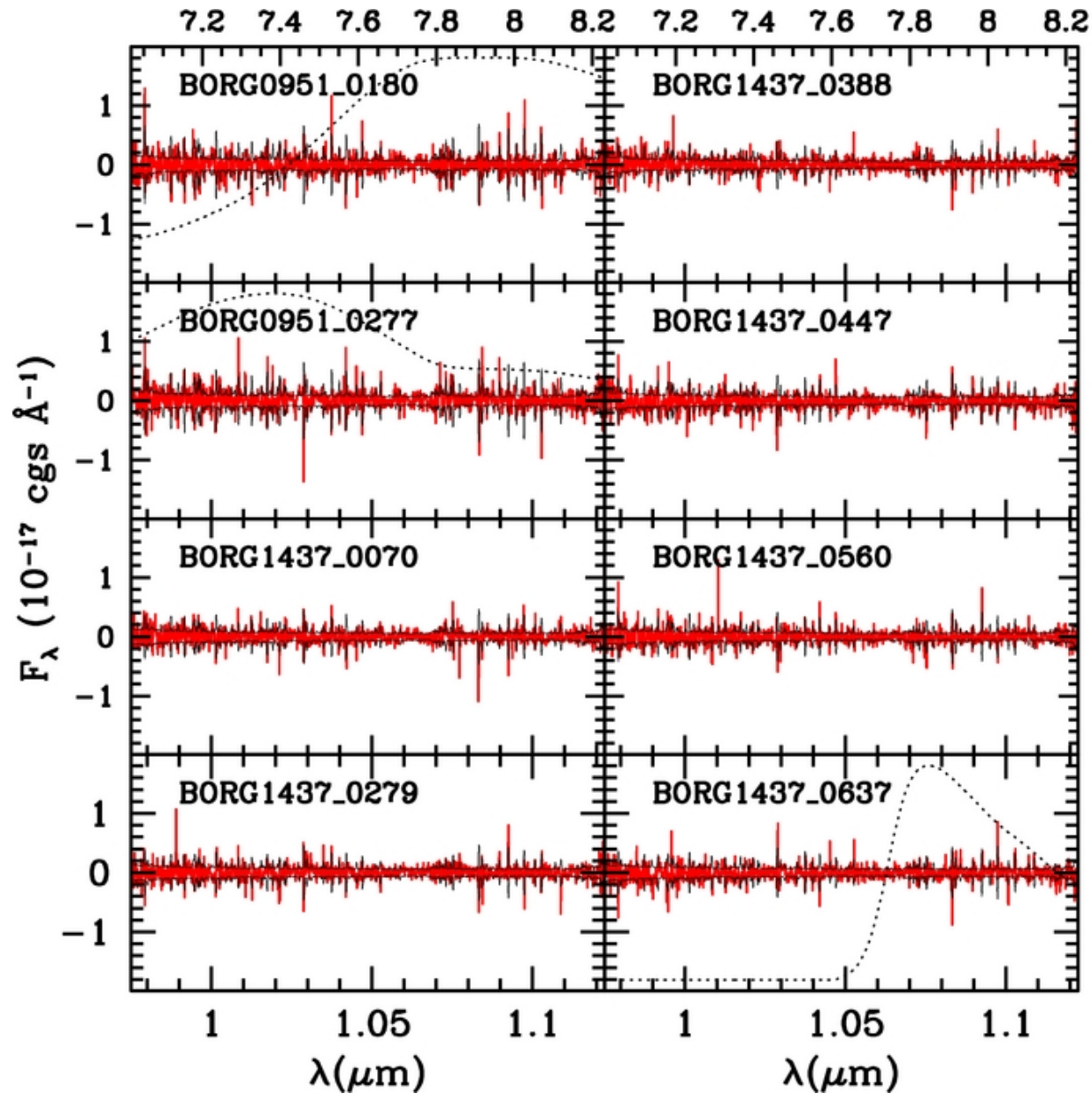
Figure 1. from The Changing Ly Optical Depth in the Range 6 < z < 9 from the MOSFIRE Spectroscopy of Y-dropouts Treu et al. 2013 ApJL 775 L29 doi:10.1088/2041-8205/775/1/L29 https://dx.doi.org/10.1088/2041-8205/775/1/L29 © 2013. The American Astronomical Society. All rights reserved.
