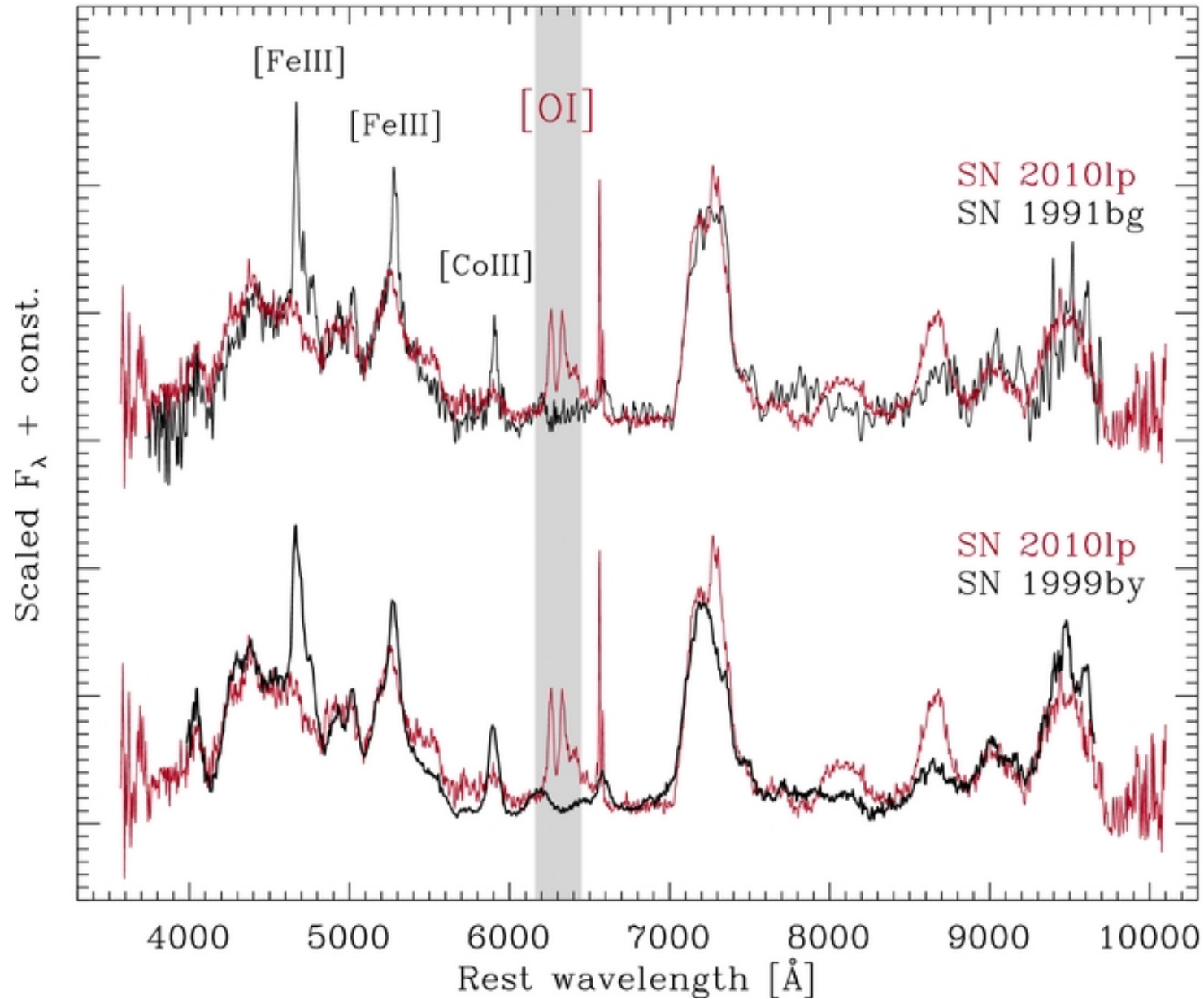
Figure 4. from [O I] 6300, 6364 in the Nebular Spectrum of a Subluminous Type Ia Supernova Taubenberger et al. 2013 ApJL 775 L43 doi:10.1088/2041-8205/775/2/L43 https://dx.doi.org/10.1088/2041-8205/775/2/L43 © 2013. The American Astronomical Society. All rights reserved.
