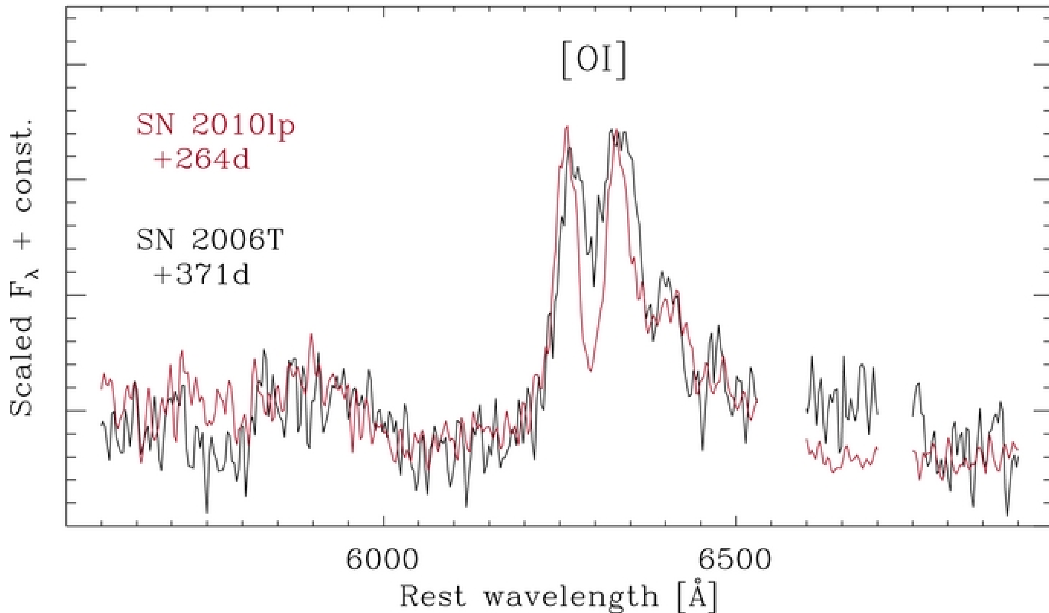
Figure 3. from [O I] 6300, 6364 in the Nebular Spectrum of a Subluminous Type Ia Supernova Taubenberger et al. 2013 ApJL 775 L43 doi:10.1088/2041-8205/775/2/L43 https://dx.doi.org/10.1088/2041-8205/775/2/L43 © 2013. The American Astronomical Society. All rights reserved.
